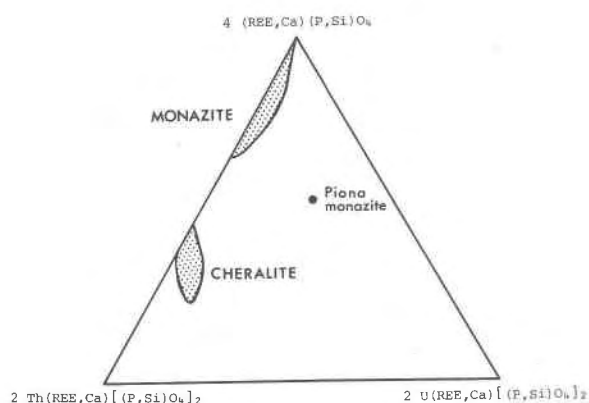
Fig. 1. Monazite, cheralite, and the Piona mineral plotted as atomic proportions in the upper half of the (\text{REE,Ca})(\text{P,Si})\text{O}_4 - \text{Th}(\text{P,Si})\text{O}_4 - \text{U}(\text{P,Si})\text{O}_4 diagram.
