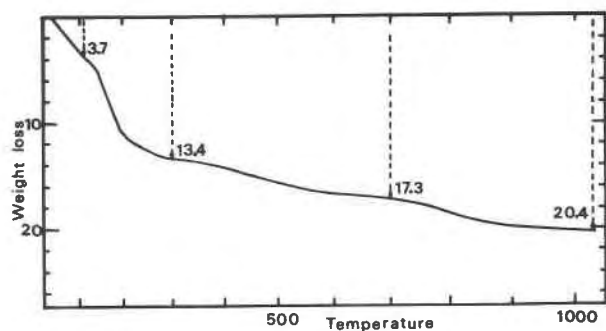
Fig. 2. Thermogravimetric curve of rancieite, 5°C/min. Weight loss as percentage of weight at 25°C, temperature °C.
