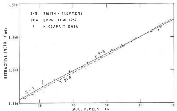
Fig. 1. Refractive index \alpha'_{001} of Kiglapait plagioclase feldspars, compared to the Smith-Slemmons curve (S-S, full line) and the curve of Burri et al. (BPW, dashed line).
