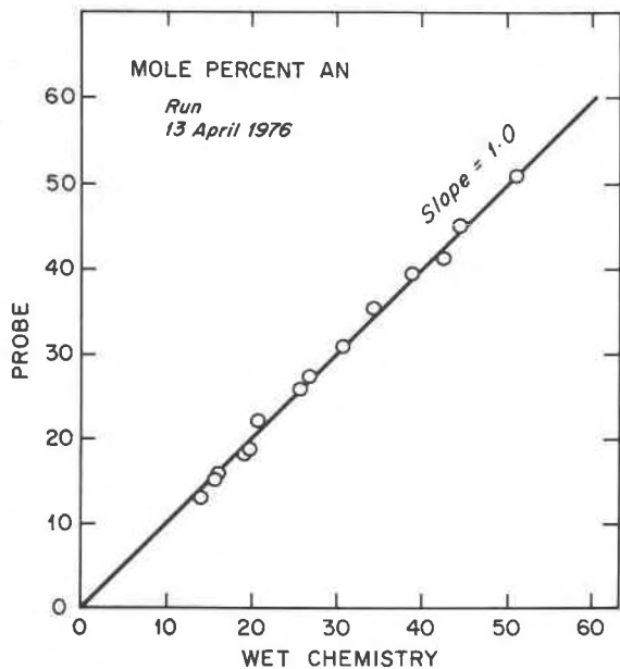
Fig. 2. Results of rapid electron probe analyses (averages of 10 grains per sample) compared to bulk chemical analyses. Circle radius is 0.9 percent An.
