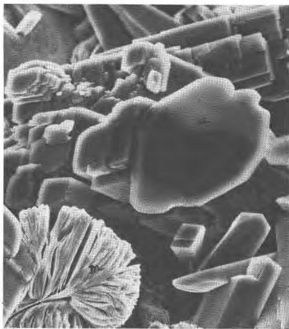
Fig. 4. Abelsonite (a) with authigenic orthoclase (o) and micaceous mineral (m) (Wosco). Scanning electron micrograph, 800 \times .
