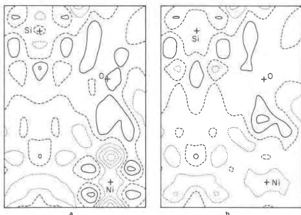
Fig. 2. Partial section of the difference electron density for \gamma - \text{Ni}_2\text{SiO}_4 through the plane y = x . Contours are at intervals of 0.2 e/\text{Å}^3 with the zero contour dashed and negative values dotted. Part (a) is for an anisotropic refinement and (b) is for a model with anharmonic terms for nickel. Atomic positions are labeled.
