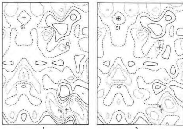
Fig. 3. Partial section of the difference electron density for \gamma -Fe 2 SiO 4 through the plane y = x . See legend of Fig. 2.
