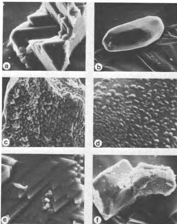
Fig. 1. (a) Octahedral cast of Fo_{92} olivine from the 0.43 ct. diamond. The inclusion is about 0.1 mm in length. (b) One of the three almandine-rich garnets from the 0.45 ct. diamond. Its length is about 0.06 mm. Their surfaces contained multitudes of hillock-like irregularities. A 10,000 \times view of the latter on the garnet shown is illustrated in (d). (c) 4000 \times view of the general octahedral topography of the outward-facing chromite layer on the chromium-rich garnet from the 0.5 ct. diamond trimineralic inclusion. (e) A restricted 20,000 \times view of the chromite. (f) The bimineralic inclusion composed of an octahedral cast of Fo_{92} olivine (left) and a crystal of pyrrhotite (attached homogeneous crustaceous residue of Fe and Ni oxides with a hexagonal shape on the right) from the 0.5 ct. diamond. The width of this inclusion is about 0.06 mm.
