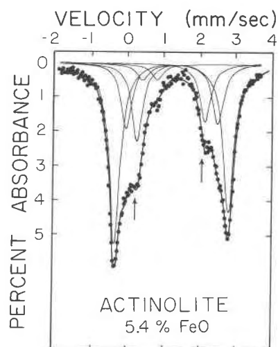
Fig. 4. Mössbauer spectrum of an actinolite from Vermont taken at 77 K, showing the increased peak separation. The FeO content represents only \text{Fe}^{2+} , and the arrows mark the locations of the inner \text{Fe}^{2+} peaks in the tremolite spectrum in Fig. 1.
