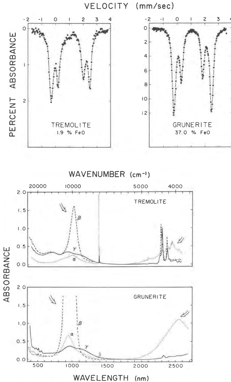
Fig. 1. Mössbauer and electronic absorption spectra of a tremolite (sample 1) from the Malagasy Republic (after Goldman and Rossman, 1977) and a grunerite (sample 2) from Canada taken at room temperature. \text{Fe}^{2+} in the M(4) sites of these amphiboles is suggested to produce the intense electronic absorption band near 1000 nm in \beta polarization and 2500 nm in \alpha polarization, and the inner quadrupole doublet in the Mössbauer spectra. The FeO value represents only \text{Fe}^{2+} . The electronic absorption spectra of tremolite and grunerite represent crystal thicknesses of 1.0 and 0.1 mm, respectively.
