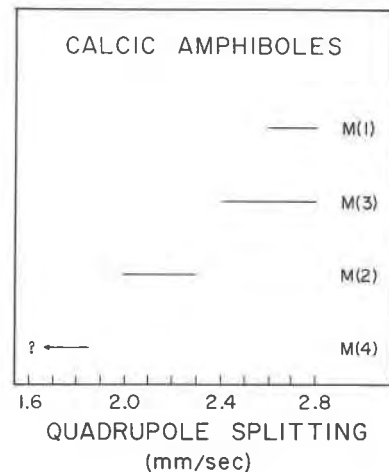
Fig. 7. Summary of the values of quadrupole splitting for Fe^{2+} in calcic amphiboles. The lower values in each range for Fe^{2+} in the M(1), M(2) and M(3) sites represent samples having more Al and Fe^{3+} .
