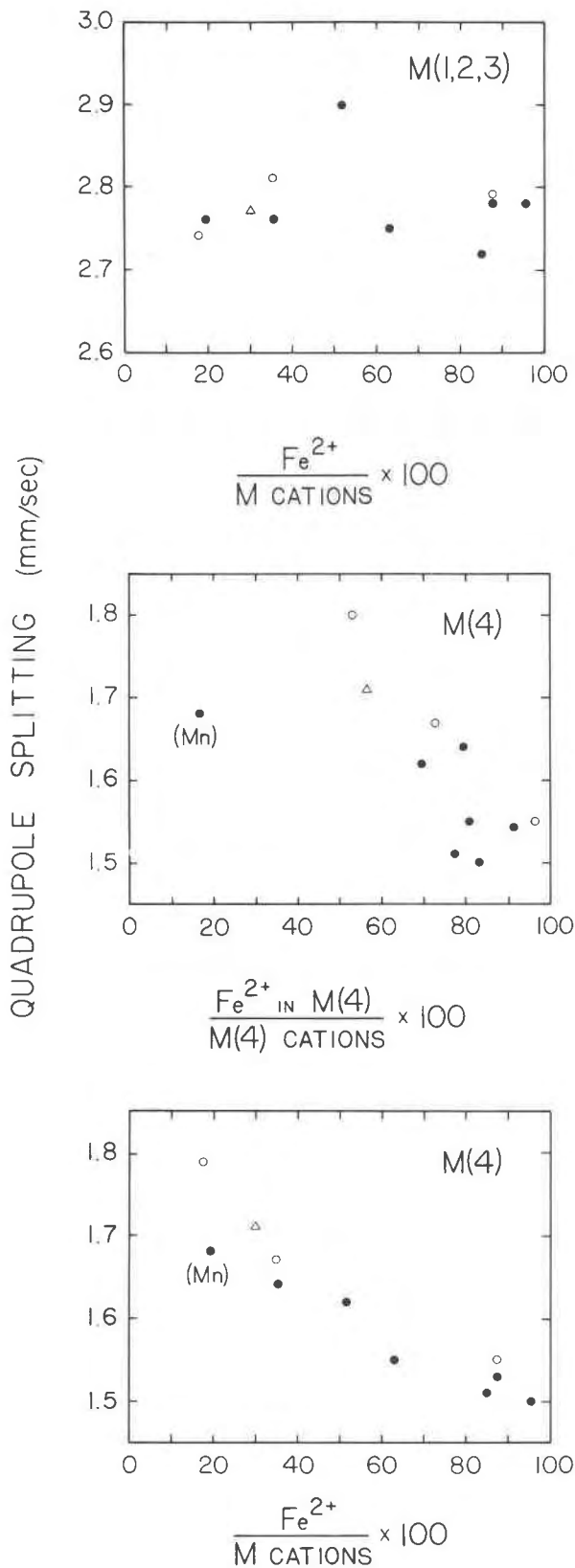
Fig. 2. Variations in the quadrupole splitting at room temperature in the cummingtonite-grunerite series.
