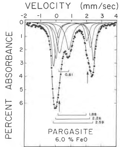
Fig. 6. Mössbauer spectrum of a pargasite from Washington taken at room temperature. The FeO content represents only Fe^{2+} , and the arrows mark the locations of the inner Fe^{2+} peaks in the tremolite spectrum in Fig. 1. The electronic absorption spectra of this sample indicate the presence of Fe^{2+} in the M(4) site.
