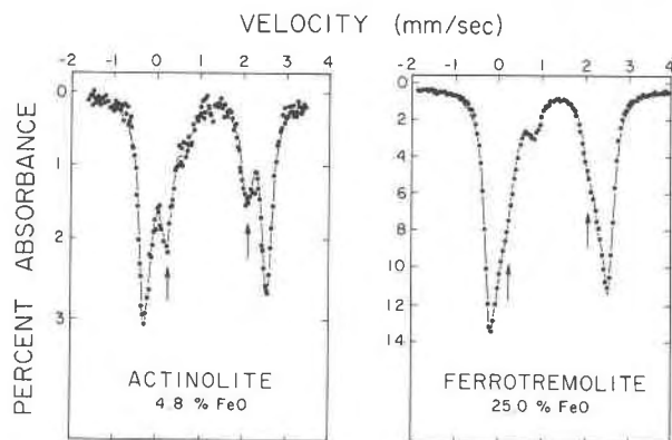
Fig. 3. Mössbauer spectra of an actinolite from California and a ferrotremolite from Minnesota taken at room temperature, which show that as the \text{Fe}^{2+} content (given as FeO) increases, the relative intensity of the inner \text{Fe}^{2+} doublet is reduced. The arrows mark the locations of the inner \text{Fe}^{2+} peaks in the tremolite spectrum in Fig. 1.
