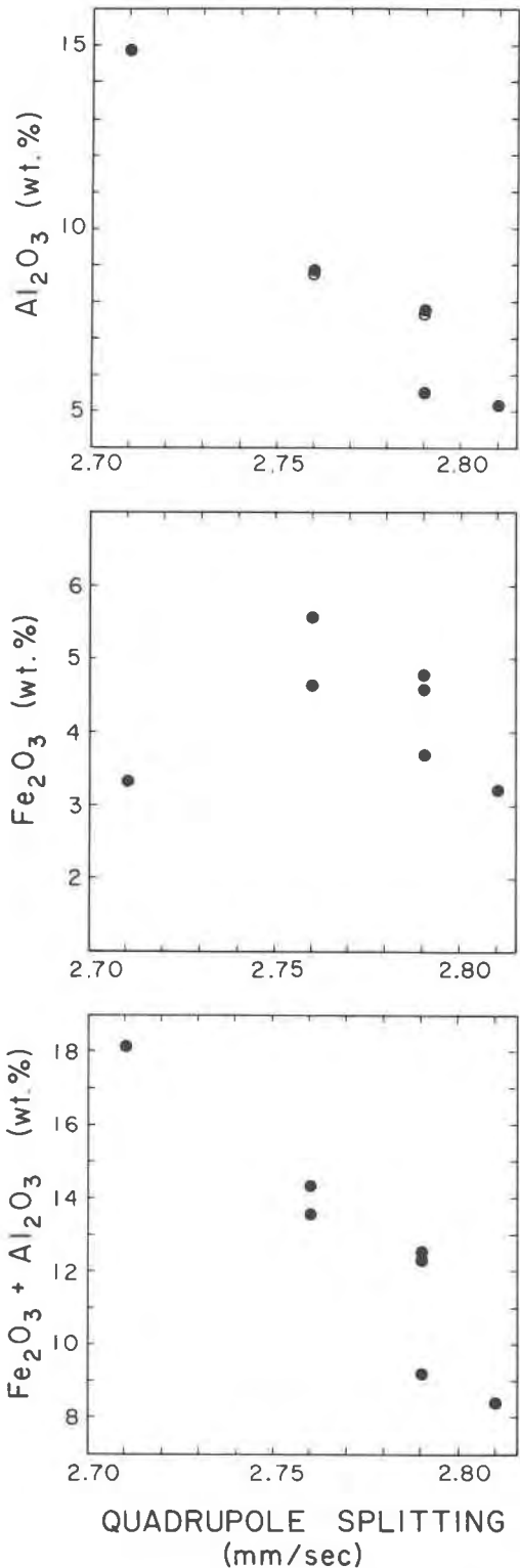
Fig. 5. Correlations between the quadrupole splitting of the outer Fe^{2+} doublet and the Al_2O_3 and Fe_2O_3 contents in the hornblendes reported by Bancroft and Brown (1975). Chemical data are from Dodge et al. (1968) and Burns and Greaves (1971).
