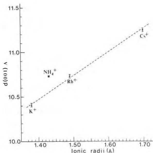
Fig. 2. Spacing of (001) for assumed 1M polymorphs of synthetic dioctahedral micas as a function of the ionic radius of the interlayer cation.
