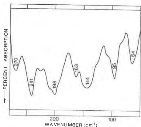
Fig. 5. The far infrared absorption spectrum of synthetic Cs-mica.
