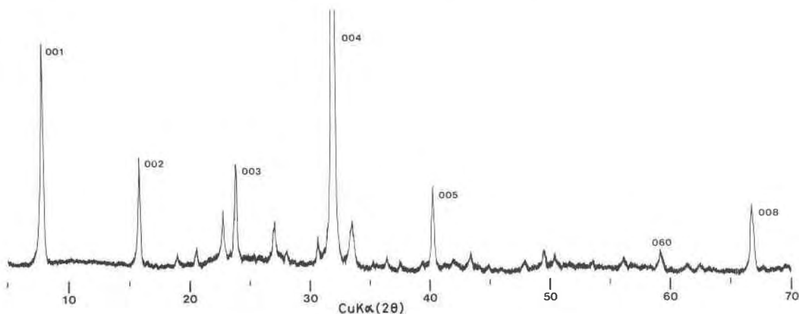
Fig. 1. X-ray powder pattern of synthetic Cs-mica.
