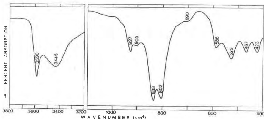
Fig. 4. The infrared absorption spectrum of synthetic Cs-mica.
