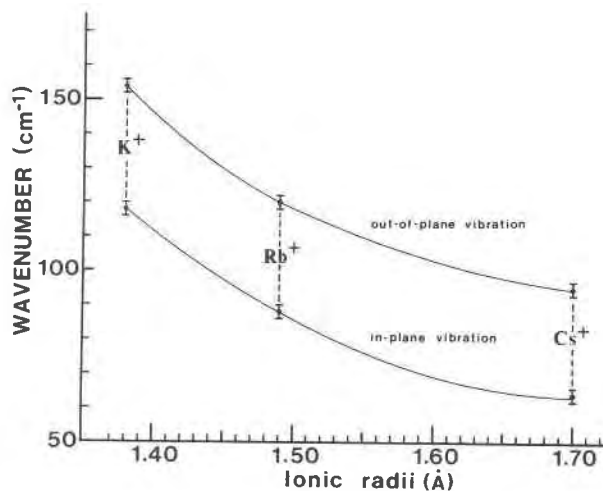
Fig. 6. The relation between stretching vibrations of alkali cation-oxygen and the ionic radius of the interlayer alkali cation.
