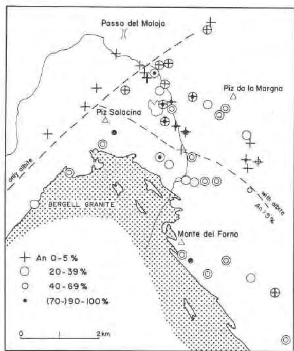
Fig. 1. Map illustrating plagioclase compositions in amphibolites around the NE contact zone of the Bergell granite (Central Alps).
