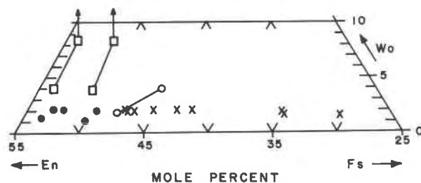
Fig. 1. Composition of clinohypersthene (crosses) and orthopyroxenes (full circles) from Ravensworth, N.S.W. Open squares and open circles represent coexisting orthopyroxenes and pigeonites from the Weiselberg and Mull andesites respectively [data from Nakamura and Kushiro (1970) and Virgo and Ross (1973)]. The upward arrows indicate coexisting augite.
