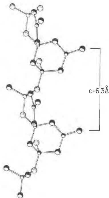
Fig. 2. The three-tetrahedral-repeat pentaborate [B_3O_{11}]^{7-} chain in hilgardite parallel to the c axis.
