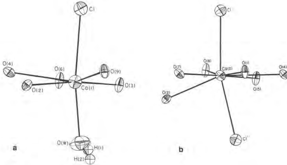
Fig. 5. The [Ca(1)O 6 Cl(H 2 O)] pentagonal bipyramid (a), and [Ca(2)O 6 Cl 2 ] hexagonal bipyramid (b) in hilgardite, showing ellipsoids of thermal vibration.
