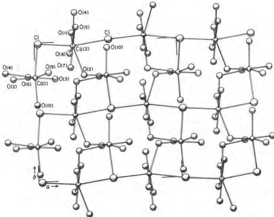
Fig. 6. The calcium polyhedral sheet in hilgardite.
