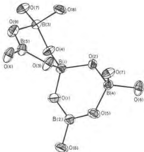
Fig. 1. A view of the [B_5O_{12}]^{9-} polyanion in hilgardite, showing the ellipsoids of thermal vibration.
