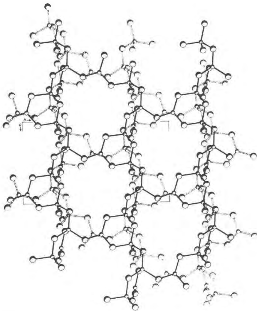
Fig. 4. A view of the pentaborate framework in hilgardite down the a axis. The borate sheet between a \sim 0.0 and \sim 0.5 is shown in full lines; the sheet between a \sim 0.5 and \sim 1.0 shown in dotted lines. Note the open channels parallel to the a axis, which are occupied by Ca(2) atoms (not shown).
