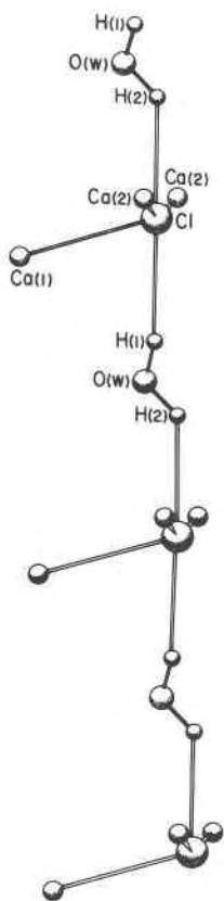
Fig. 7. The hydrogen bonded quasi-linear Cl...H-O-H...Cl chain in hilgardite, parallel to the c axis. Note the five-fold trigonal bipyramidal coordination of the chlorine atom.
