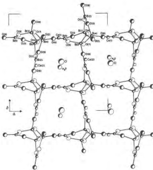
Fig. 3. The zeolite-type [B_5O_9]^{3-} framework in hilgardite viewed down the c axis. Note the chlorine atoms and the water molecules occurring within the channels parallel to c .
