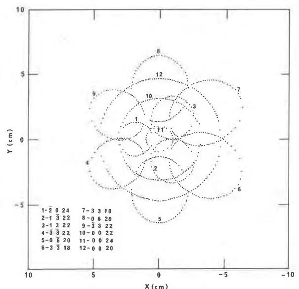
Fig. 2. Calculated pseudo-Kossel curves for talc. Crystal-film = 63 mm. Crystal-target = 5 mm. Radiation = CuK.
