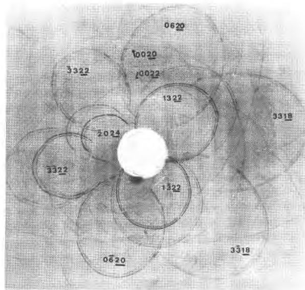
Fig. 1. Double exposure pseudo-Kossel photograph of a talc crystal (CuK radiation).
