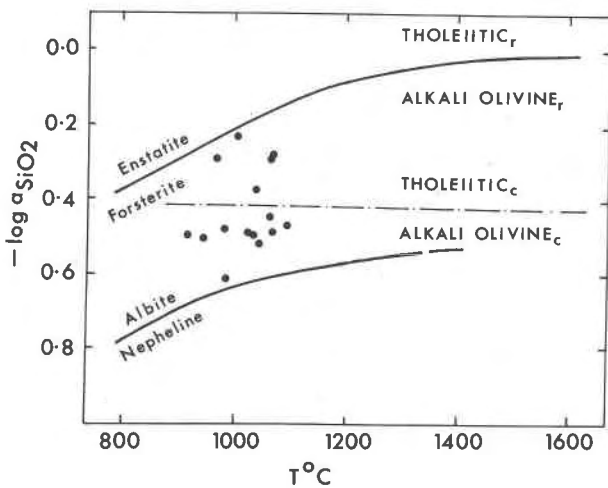
Fig. 1. T vs. -\log a_{\text{SiO}_2}/\text{melt} showing 2 buffer reactions, the extrapolated (dash-dot) curve for the critical plane eutectic composition, and the data for -\log a_{\text{SiO}_2}/\text{melt} at T for SRP lavas from Stout and Nicholls (1977). The subscripts r and c refer to buffer-reaction and critical-plane classification criteria respectively.
