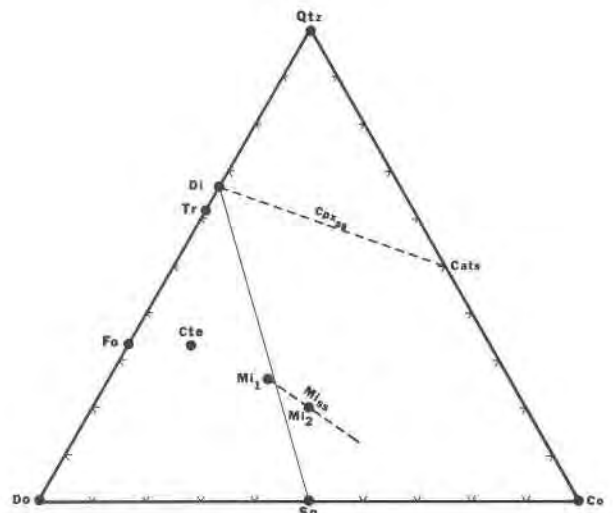
Fig. 2. Composition of model phases in the system \text{CaO-MgO-SiO}_2\text{-Al}_2\text{O}_3\text{-CO}_2\text{-H}_2\text{O} projected from calcite, \text{CO}_2 , and \text{H}_2\text{O} onto the plane dolomite-quartz-corundum. Abbreviations and compositions: Qtz = quartz; Co = corundum; Do = dolomite; Fo = forsterite; Tr = tremolite; Di = diopside; Cats = calcium Tschermak's pyroxene; Sp = MgAl-spinel; Cte = chlorite [\text{Mg}_5\text{Al}_2\text{Si}_3\text{O}_{10}(\text{OH})_8] ; \text{Mi}_{\text{ss}} = range of clintonite solid solution; \text{Mi}_1 = \text{CaMg}_2\text{Al}_4\text{Si}_{14}\text{Al}_2\text{O}_{10}(\text{OH})_2 ; \text{Mi}_2 = \text{CaMg}_2\text{AlSiAl}_3\text{O}_{10}(\text{OH})_2 .
