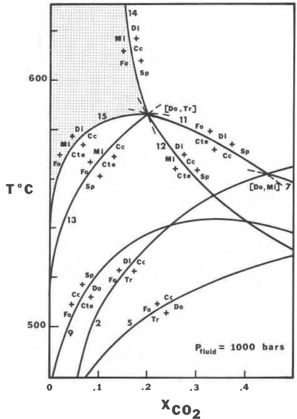
Fig. 7. Temperature-fluid composition diagram for a total pressure of 1000 bars, showing approximate locations of stable reactions involved in the formation of clintonite. Shaded area shows the stability field for clintonite-bearing assemblages observed in the Boulder aureole.
