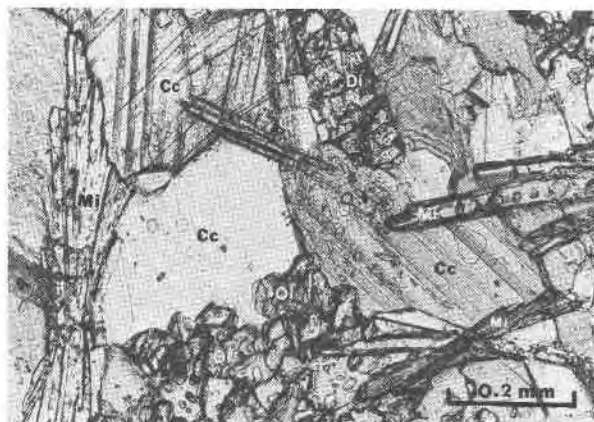
Fig. 3. Photomicrograph of the assemblage calcite (Cc)-olivine (Ol)-diopside (Di)-clintonite (Mi).
