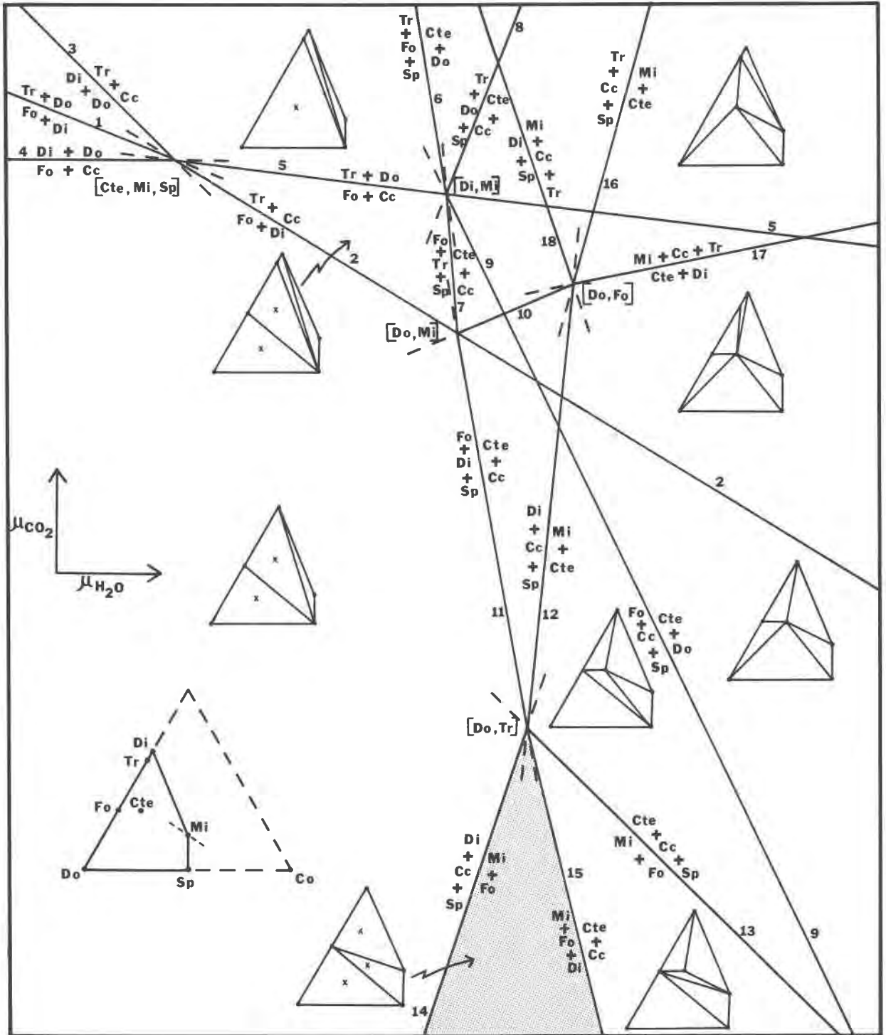
Fig. 6. \mu_{\text{CO}_2} vs. \mu_{\text{H}_2\text{O}} diagram of end-member discontinuous reactions. Invariant point notation is that of phases absent. Shaded area shows the stability field for clintonite-bearing assemblages observed in the Boulder aureole. Chemographic diagrams are projections from \text{CaCO}_3 , \text{CO}_2 , and \text{H}_2\text{O} . X indicates observed 3-phase (+ calcite) assemblages.
