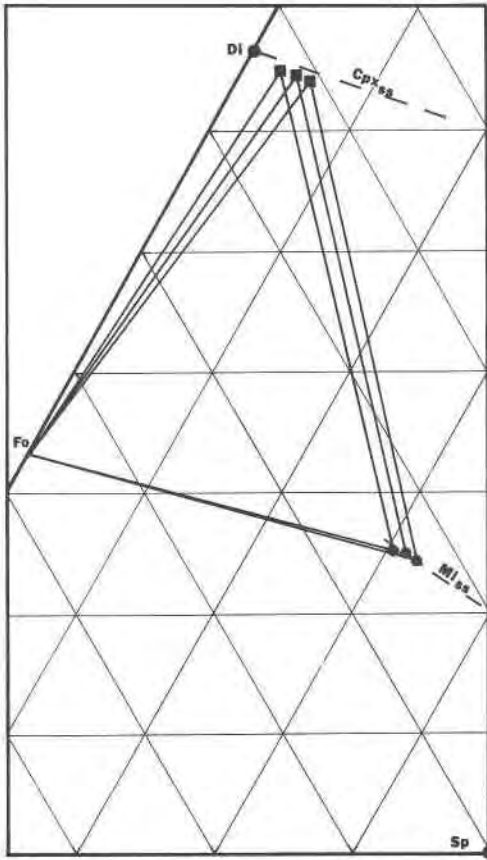
Fig. 4. Compositions of coexisting clinopyroxene and clintonite projected onto a portion of the plane \text{SiO}_2\text{-MgO-Al}_2\text{O}_3 .
