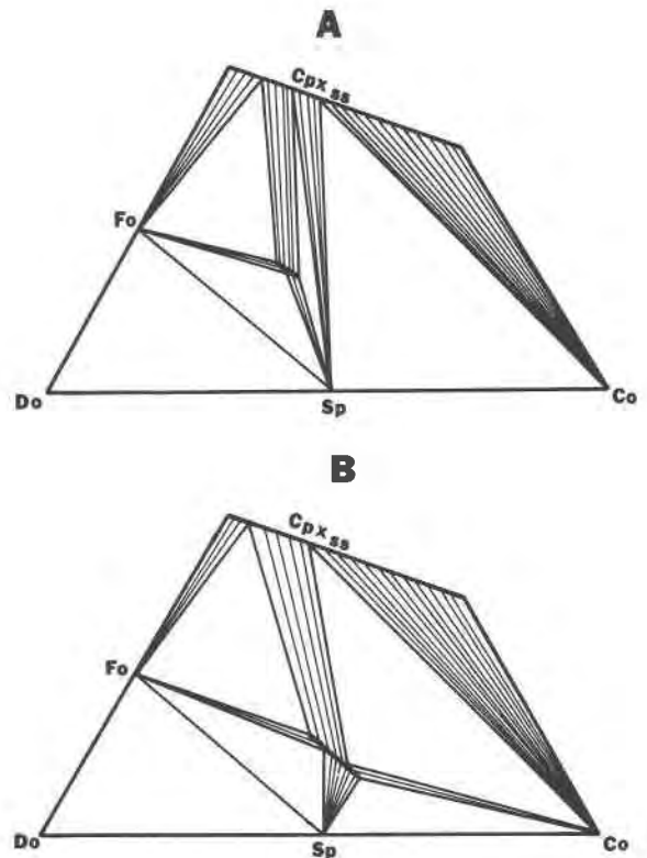
Fig. 5. (A) Configuration of 3-phase triangles resulting from reaction (a) \text{Fo} + \text{Di} + \text{Sp} + \text{Cc} + \text{H}_2\text{O} = \text{Mi} + \text{CO}_2 . (B) Configuration of 3-phase triangles resulting from reaction (b) \text{Di} + \text{Cc} + \text{Sp} + \text{H}_2\text{O} = \text{Fo} + \text{Mi} + \text{CO}_2 .
