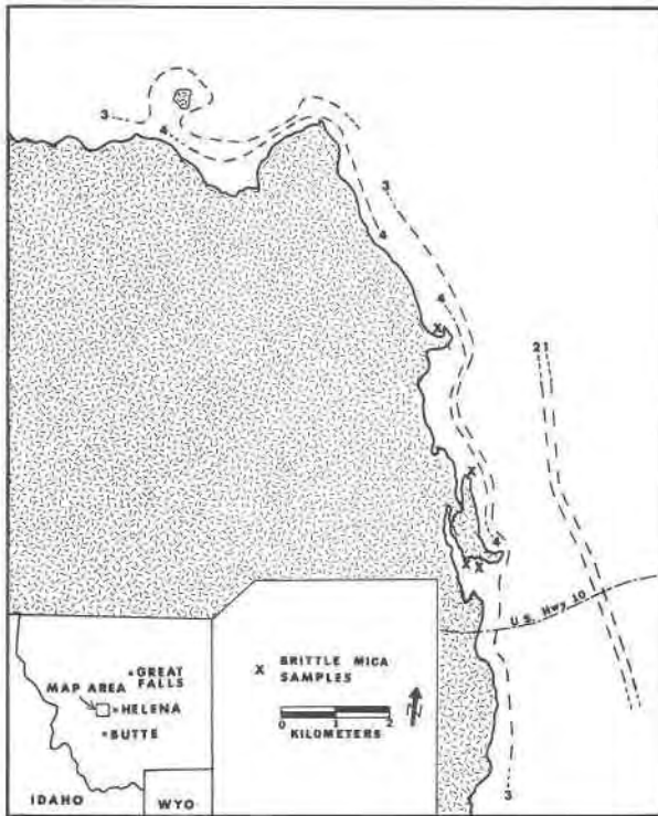
Fig. 1. Outline geologic map of the northernmost portion of the Boulder batholith showing the location of clintonite-bearing samples. Numbered isograds described in detail by Rice (1977) include: (1) first appearance of tremolite and phlogopite; (2) first appearance of diopside in silica-saturated bulk compositions; (3) appearance of olivine + spinel and simultaneous disappearance of calcic amphibole + dolomite; (4) appearance of diopside + calcite + spinel.
