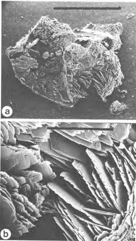
Fig. 1. Scanning electron microscope pictures of cluster of schoderite from Arkansas. (a) Overall dimensions 0.9 mm, bar length 0.5 mm. (b) Detail of lower part of cluster, bar length 0.1 mm.
