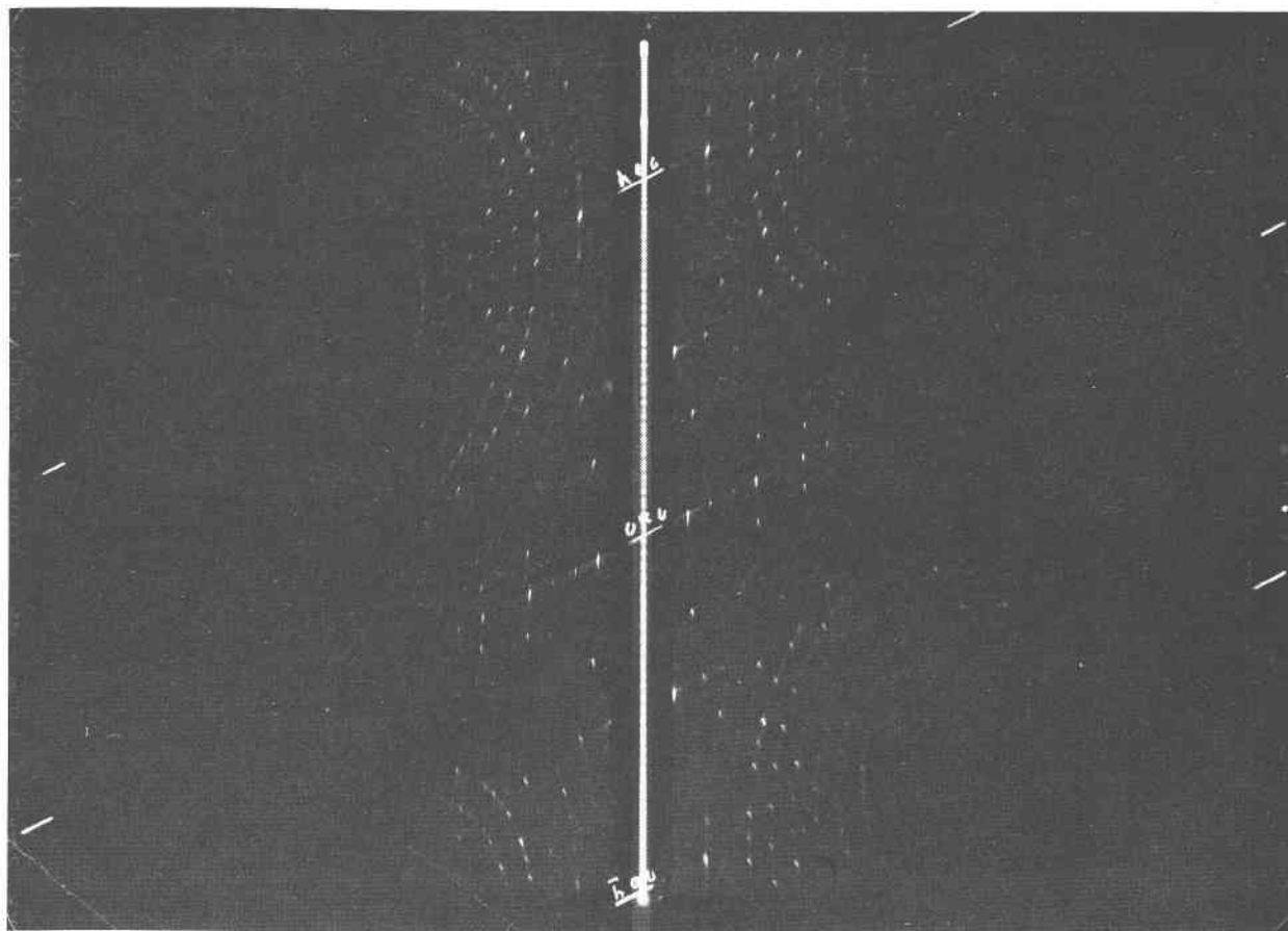
Fig. 5. hk0 Weissenberg pattern of schoderite from Arkansas. Notice diffuseness of spots with k even and slight streaking in b^* direction. There are no diffraction spots at 2\theta angles greater than 60^\circ .
