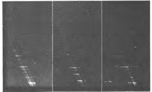
Fig. 8. Schoderite from Arkansas; 0k0 loci on three Weissenberg films, Cu-radiation, no filter. Left, \times 1 , #12, untreated; center, \times 1 , #10, heated to 31°C, partly dehydrated; right, \times 1 , #10, rehydrated.
