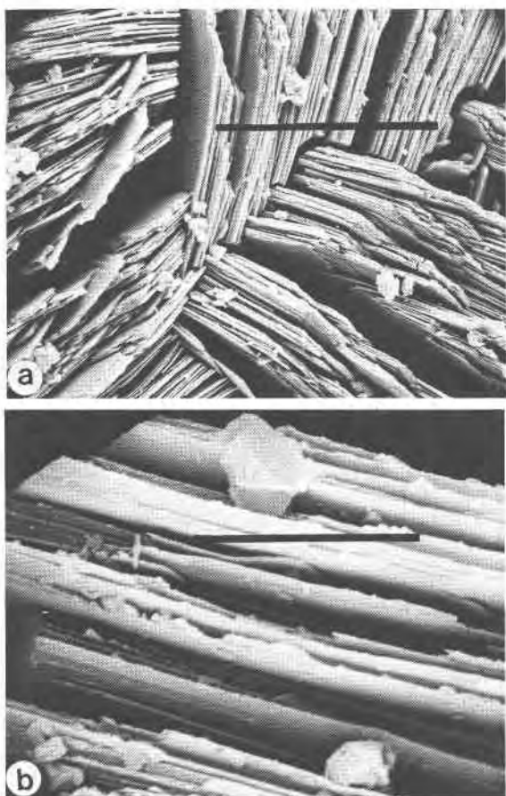
Fig. 3. (a) Finer detail of junction seen in Fig. 2b; length of bar 0.05 mm. (b) Thin, diverging platelets from right central part of Fig. 3a; length of bar 0.005 mm.
