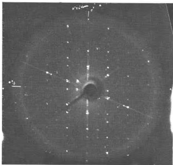
Fig. 6. h0l precession pattern of schoderite from Arkansas. Precession angle 25^\circ , Cu radiation, no filter, beam normal to cleavage. \beta , 92^\circ , can be read directly from pattern.
