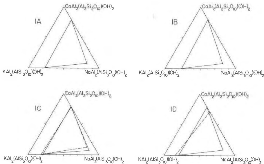
Fig. 1. Compositions of coexisting margarite + paragonite + muscovite in terms of end-member white micas. (A) Specimen P-1, using margarite and paragonite analyses done on the U.W. probe and muscovite analyzed on the U.M. probe. (B) Specimen P-1, using only analyses done on the U.M. probe. (C) Specimen P-2. Solid lines used for analyses done on the U.W. probe; dashed lines used for analyses done on the U.M. probe. (D) Plot showing average end-member values for margarite, paragonite, and muscovite in specimens P-1 and P-2 (solid lines). Average includes U.W. and U.M. analyses. Dashed line shows the margarite–muscovite pair reported by Guidotti and Cheney (1976).
