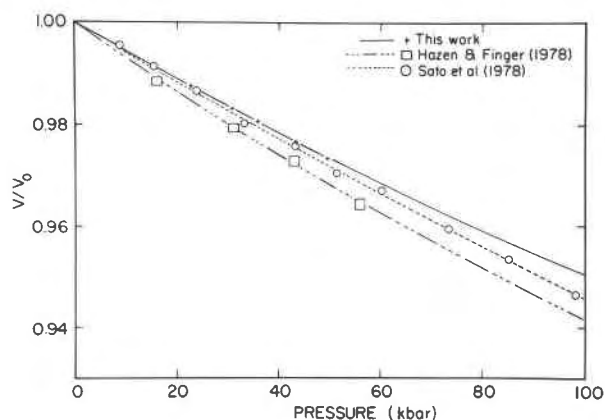
Fig. 1. V/V_0 vs. pressure for pyrope. Curves represent third-order Birch-Murnaghan equation of state for each of the sets of data.
