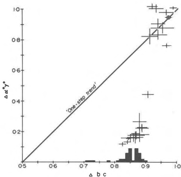
Fig. 1. \Delta bc vs. \Delta\alpha^*\gamma^* for 65 K-feldspars and one albite in perthitic intergrowth (circled, sample 66). Symbols for triclinic samples extend one standard deviation from the mean. Distribution of monoclinic samples is shown by the histogram; the smallest step represents one sample.
