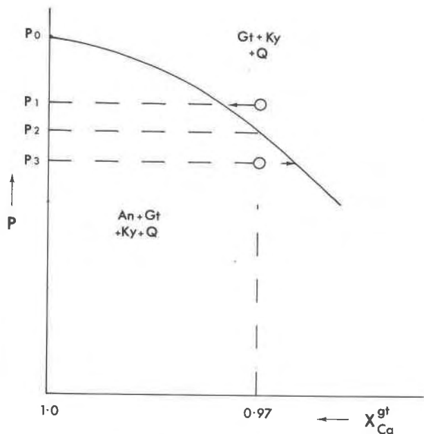
Fig. 1. A garnet solid solution of X_{Gr} = 0.97 would be in equilibrium with anorthite, kyanite and quartz at P_2 . This pressure is experimentally bracketed by demonstrating increasing X_{Ca}^{gt} at P_1 and decreasing X_{Ca}^{gt} at P_3 .
