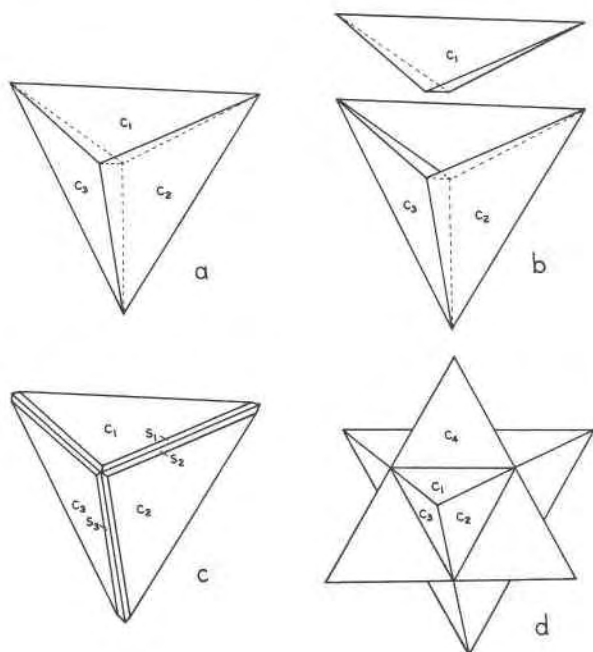
Fig. 1. Idealized drawings of crystals of okanoganite. The individuals in each fourling are differentiated by the subscripted numbers. Forms present are c\{0001\} and s\{10\bar{1}4\} . Drawing b shows a fourling with one of the individuals separated to better show the twinning relationship.
