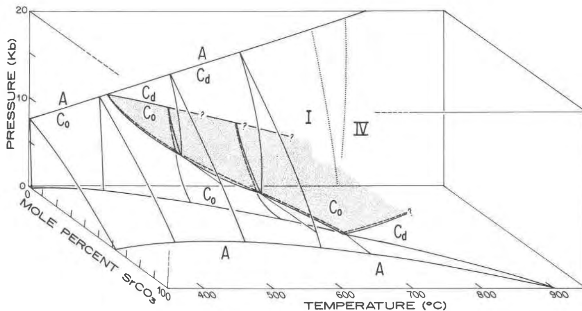
Fig. 6. P - T - X diagram of phase relations in the system \text{CaCO}_3 - \text{SrCO}_3 . Surfaces bounding the two-phase field for ordered and disordered calcite are indicated by shading. Data on rear face from Johannes and Puhani (1971), Mirwald (1976), and after Goldsmith and Newton (1969); data on bottom face after Chang (1965). Field labels as for Figs. 1 and 2.
