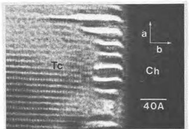
Fig. 18. An unusual talc-chesterite interface. The image is uninterpretable in terms of normal biopyribole structure and may result from twisting of the talc sheets near the interface.
