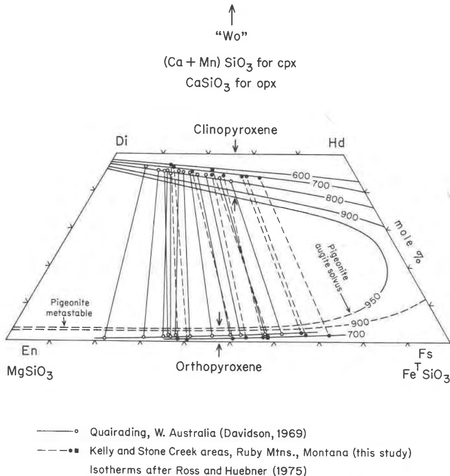
Fig. 8. Pyroxene pairs from the Ruby Range (single, not averaged, analyses plotted) compared with those from the Quairading district of Western Australia (Davidson, 1969). Superimposed is the experimentally-determined pyroxene solvus of Ross and Huebner (1975). It is assumed that Ca and Mn occupy the M2 site of clinopyroxene; the relative position of the two curves is not changed, however, if Mn is plotted with \text{Fe}^T (total iron) instead of with Ca. Ross and Huebner place a \pm 100^\circ\text{C} uncertainty on temperatures estimated by their method.
