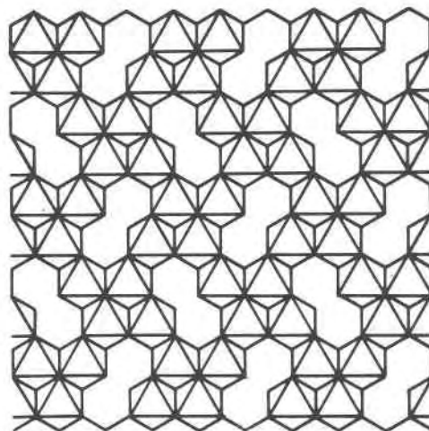
Fig. 1. A two-dimensional framework created by removing one third of the octahedra as edge-sharing pairs from a close-packed layer of octahedra.
