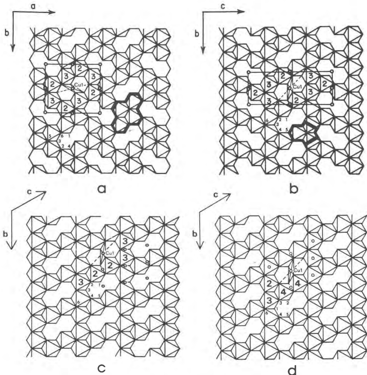
Fig. 2. The idealized frameworks of the \text{Cu}_5(\text{PO}_4)_2(\text{OH})_4 polymorphs: (a) PPM, (b) PM, (c) XPM, (d) QPM. Large numbers identify the copper polyhedra, small numbers the oxygen atom positions, and small circles the locations of inversion centers. The nature of the Cu(1) site is shown.
