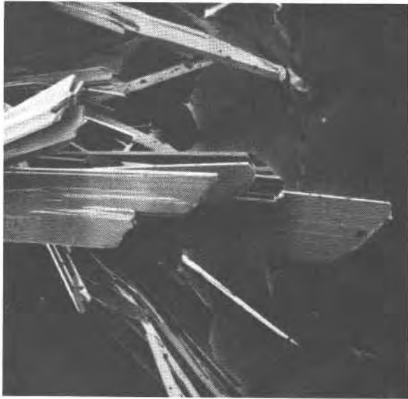
Fig. 1. Scanning electron microscope photomicrograph of ajoite showing the bladed habit. The width of the large crystal is about 0.1 mm.
