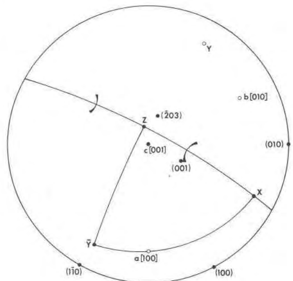
Fig. 2. Stereographic projection of optical and crystallographic elements of ajoite.
