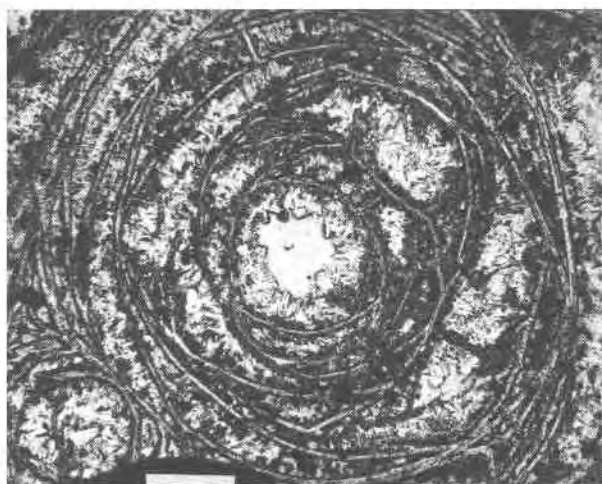
Fig. 4. Photomicrograph of altered glass from 14.2 m (plane light). Perlitic texture is preserved by deposition of montmorillonite along concentric shell-like hydration cracks. Subsequent alteration consists of deposition of clear, tabular, intermediate heulandite crystals oriented perpendicular to clay-filled hydration cracks. White bar at bottom left is 0.1 mm.
