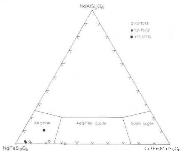
Fig. 8. \text{NaAlSi}_2\text{O}_6 - \text{NaFeSi}_2\text{O}_6 - \text{Ca}(\text{Fe},\text{Mn})\text{Si}_2\text{O}_6 ternary diagram showing variation in aegirine composition for two samples from drill core Y-2 (data from Table 6) and one sample from Y-13. Composition of aegirine from drill core Y-13 from T. E. C. Keith and M. H. Beeson (unpub. data, 1979).
