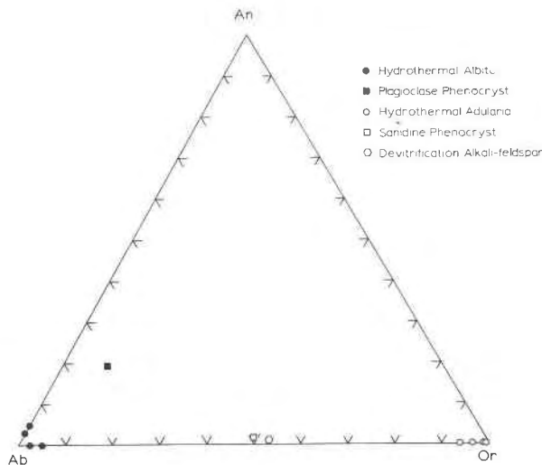
Fig. 7. An-Ab-Or ternary diagram for feldspar minerals encountered in Y-2 drill core. Data from Table 5.
