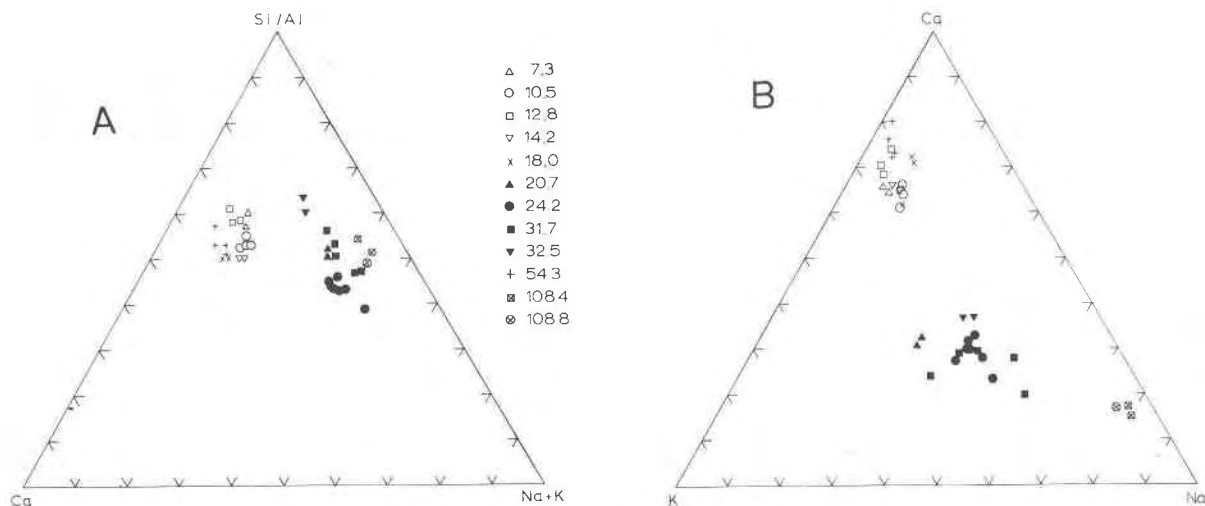
Fig. 6. (A) Ternary diagram of Si/Al-sum of divalent cations-sum of monovalent cations for heulandite-group zeolites from Y-2 drill core. Data from Table 2. Sum of divalent cations shown as Ca because no Mg, Ba, or Sr was found in any of the samples analyzed. (B) Ca-K-Na plot for heulandite-group zeolites from Y-2 drill core. Data from Table 2. Symbols same as in Figure 6(A).
