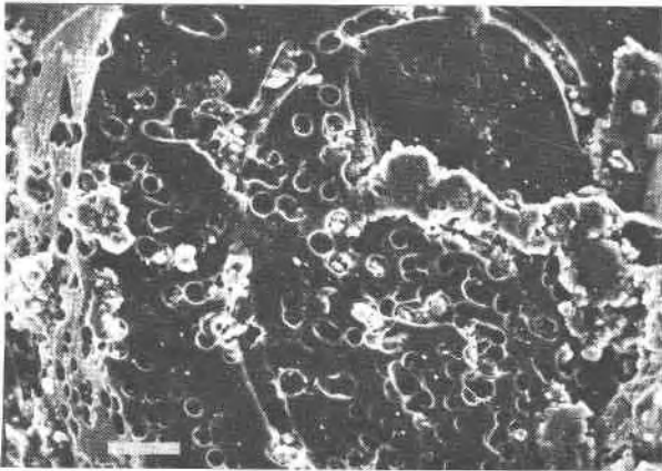
Fig. 3. Scanning electron micrograph of broken surface of obsidian grain from 26.2 m. Surface and interior of grain contain numerous shallow vesicles partly filled by clinoptilolite and montmorillonite. White bar at bottom left is 30 microns.
