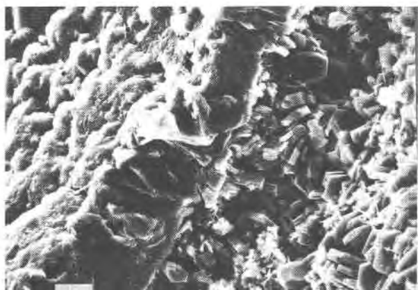
Fig. 5. Scanning electron micrograph of altered glass from 14.2 m. A montmorillonite-filled former hydration crack shown in left half of photo. Right half shows area between clay-filled hydration cracks in which tabular- or "tombstone"-shaped intermediate heulandite crystals are oriented perpendicular to remanent hydration cracks. Fibrous mordenite and clusters of montmorillonite platelets are later than the heulandite. White bar at bottom left is 10 microns. (After Bargar et al. , 1981.)
