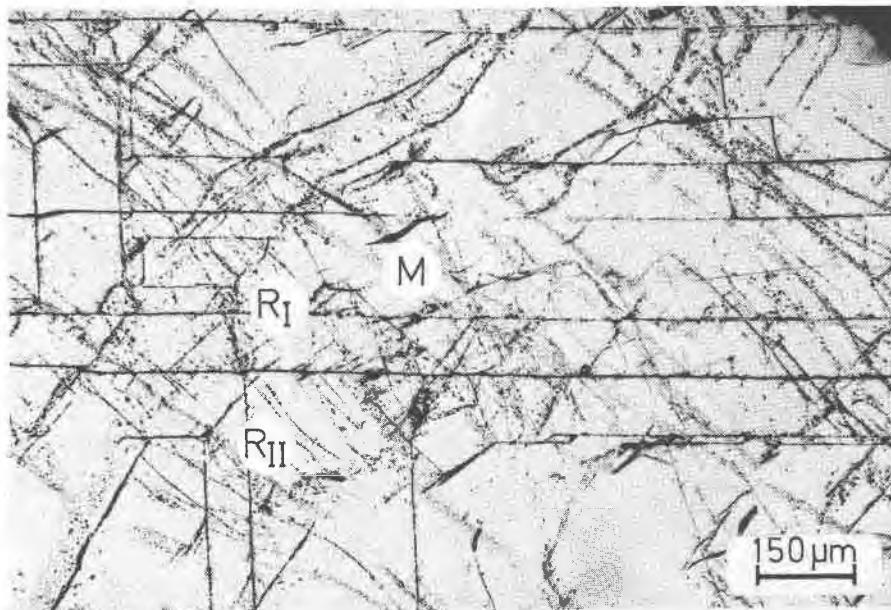
Fig. 2. Photomicrograph of linear rhombohedral cleavage fracture systems R_1 and R_{II} and of healed fissures M ; thin section cut perpendicular to the two macroscopic cleavage systems.
