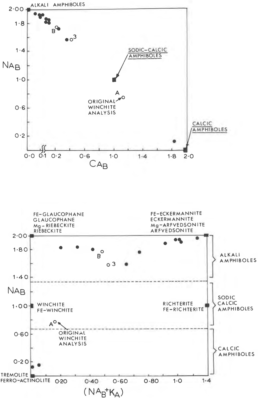
Fig. 1. Plots of representative analyses of amphiboles from Kajlidongri (Table 1). Open circles are wet-chemical analyses; solid spots, microprobe data. The sample numbered 3 is from Lahiri (1971). Only end-member amphiboles with 8 Si in the standard formula are named specifically.
