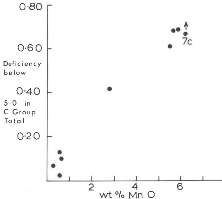
Fig. 2. Plot of Mn contents of amphiboles against the deficiency below 5.00 in the C-group total, i.e. , 5.00 minus C-group total.
