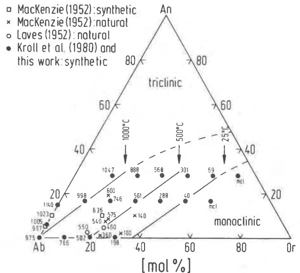
Fig. 7. Variation of T_{\text{displ}} [°C] in the ternary system Or-Ab-An. T_{\text{displ}} is indicated beside the data points. Contours drawn for 25°C, 500°C, 1000°C are based on the synthetic samples. The transition plane corresponds to T_{\text{equil}} = 1000 - 1100^\circ\text{C} . Increasing Al,Si order within topochemically monoclinic samples due to a decrease of T_{\text{equil}} lowers the plane (Kroll et al. , 1980, Eq. 3). Sources of data: Laves (1952), MacKenzie (1952), Kroll et al. (1980, Eq. 1 for T_{\text{equil}} = 1000^\circ\text{C} ), this paper: Figure 3 and 6 where T_{\text{displ}} = 1140^\circ\text{C} is taken at the intersection of the curve of the displacive transformation with the (dry) solidus curve.
