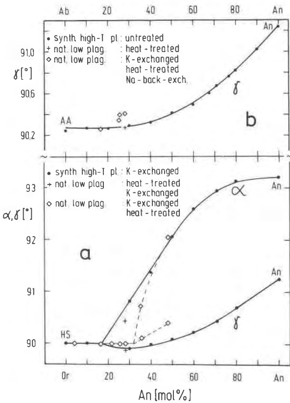
Fig. 2. (a) Variation with composition of \alpha and \gamma angles of Kroll and Müller's (1980) K-exchanged equivalents of high-temperature plagioclases (dots) plus K-exchanged and subsequently heated low plagioclases (diamonds). (b) Variation with composition of the \gamma angles of Kroll and Müller's (1980) high-temperature plagioclases (dots) plus Na-back-exchanged (K,Ca)-sanidines (diamonds).
