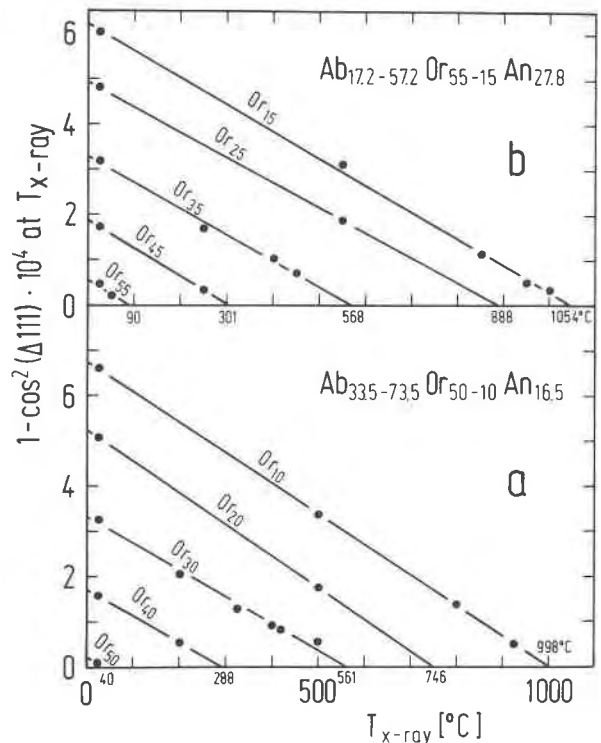
Fig. 3. Variation with temperature of the parameter 1 - \cos^2(\Delta 111) within the topochemically monoclinic series (a) Or_{10-50} Ab_{73.5-33.5} An_{16.5} and (b) Or_{15-55} Ab_{57.2-17.2} An_{27.8} . The indicated temperatures of the displacive transformation, T_{displ} , were determined from linear least-squares fitting. \Delta 111 = 4\theta(111) - 4\theta(1\bar{1}1) , CuK\alpha_1 .
