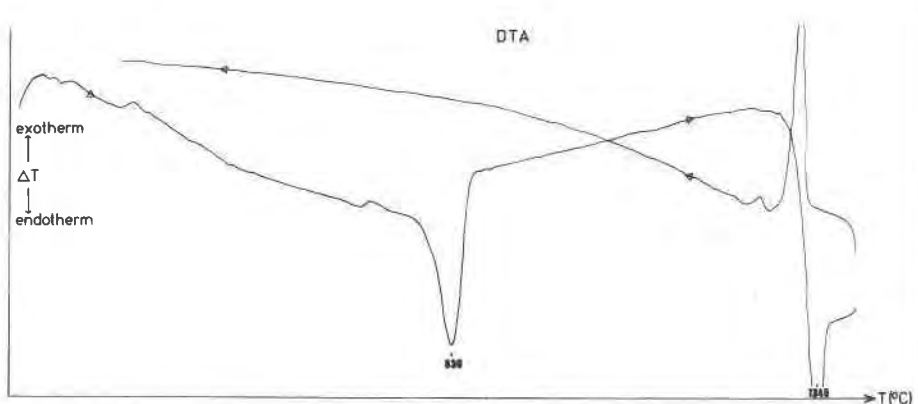
Fig. 5. DTA heating and cooling curve of karlite; dehydration occurs at 830^\circ\text{C} and melting at 1345^\circ\text{C} .
