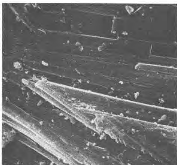
Fig. 2. SEM photograph of karlite showing the parallel and subparallel intergrowth of small fibers. Horizontal white bar is 2 \mu m .
