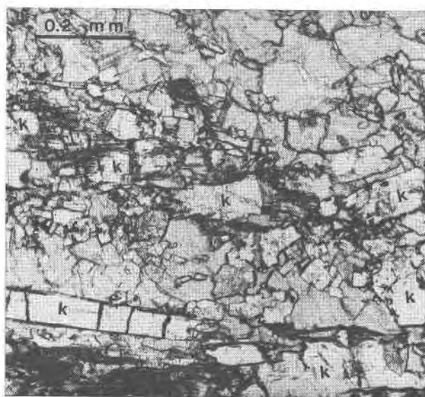
Fig. 1. Photomicrograph of karlite (k). Fig. 1a is typical of the fibrous and needle like character of the mineral. Fig. 1b shows the pseudotetragonal morphology with \{110\} and subordinate \{100\} .
