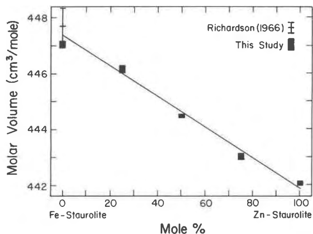
Fig. 3. Molar volume vs. composition for synthetic Fe/Zn staurolites. Symbols are 2 esd 's in height.
