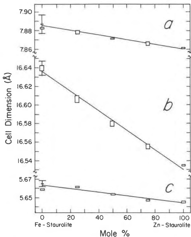
Fig. 2. Variation of lattice parameters with composition for synthetic Fe/Zn staurolites. Symbols: rectangles, this study; vertical bars, Richardson (1966). Symbols are 2 esd 's in height.
