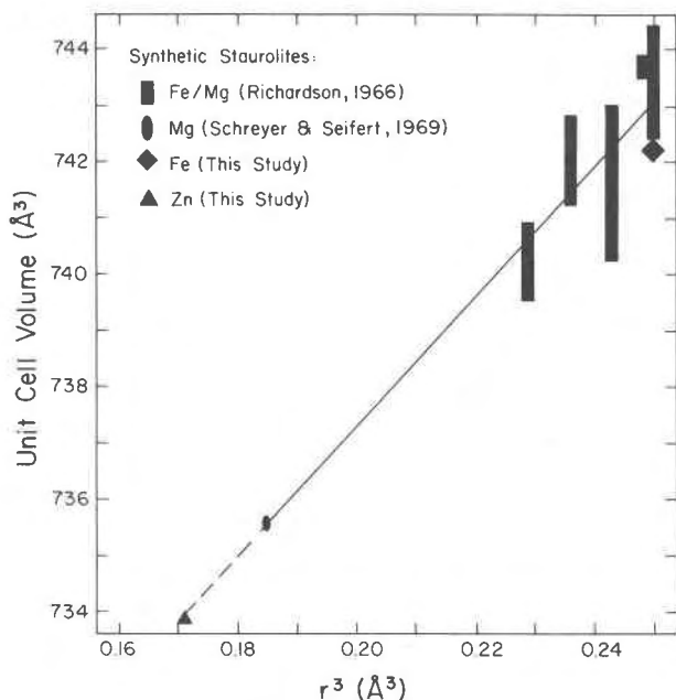
Fig. 4. Unit cell volume of synthetic Fe/Mg staurolite as a function of the cube of the mean effective ionic radius of the metal atom (Shannon, 1976). The value of r^3 for ^{IV}\text{Zn}^{2+} is determined by extrapolating the least-squares line to the observed unit cell volume of zinc staurolite (Table 1). Symbols are 2 esd 's in height.
