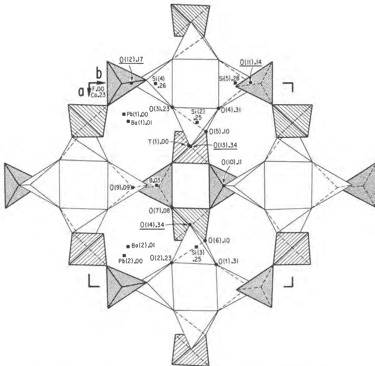
Fig. 1. Polyhedral representation of hyalotekite down [001]. The section 0 \leq z \leq \frac{1}{2} is shown. The [\text{Si}_4\text{O}_{12}] ring is not shaded, the \text{T}(1) ( = \text{Si}_{3/4}\text{Be}_{1/4}\text{O}_4 ) tetrahedra are ruled and the \text{BO}_4 tetrahedra are stippled. Heights are given as fractional coordinates in z . The asymmetric unit in Table 2 is labelled. Terminal oxygens are underlined.
