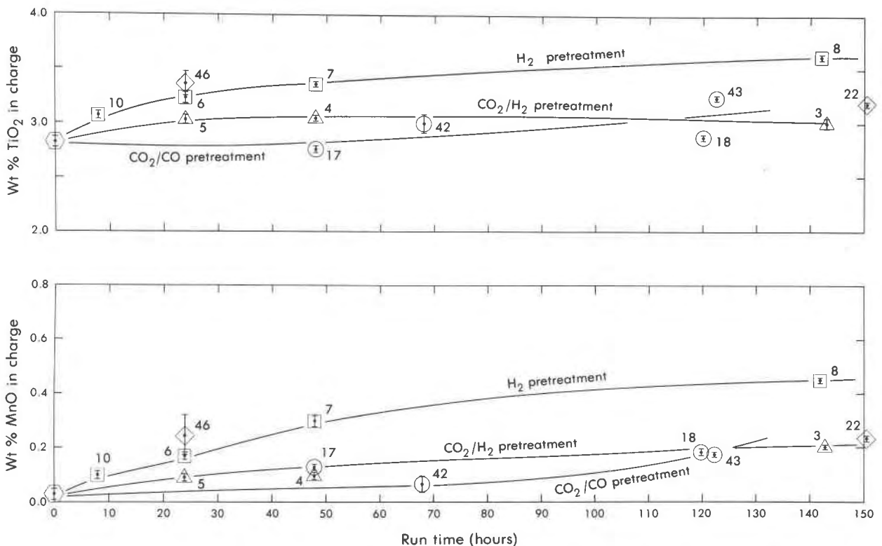
Fig. 5. Wt.% TiO 2 (above) and wt.% MnO (below) vs. time in charges run in electromagnet-grade iron crucibles pretreated in H 2 (squares), CO 2 -H 2 (triangles), CO 2 -CO (circles) and untreated (diamonds). The composition of the starting mixture (Table 3) is represented by a hexagon. Each point represents an average of three to five analyses and error bars define one standard deviation about the mean. Run numbers correspond to those in Table 4.
