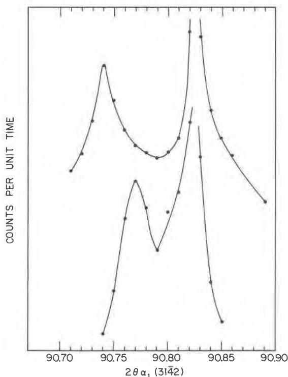
Fig. 2. Paired reflections of \alpha_1 ( 3\bar{1}42 ) in chalcedony with 1:1 oscillatory zoning.
