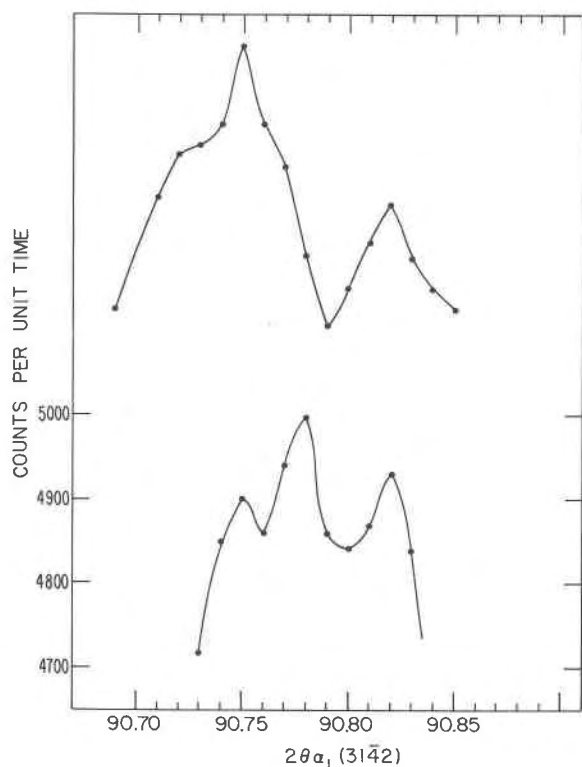
Fig. 3. Multiple peaks in \alpha_1 ( 3\bar{1}\bar{4}2 ) in a density fraction with d \sim 2.597 (above), and in a bulk sample of randomly zoned chalcedony (below).
