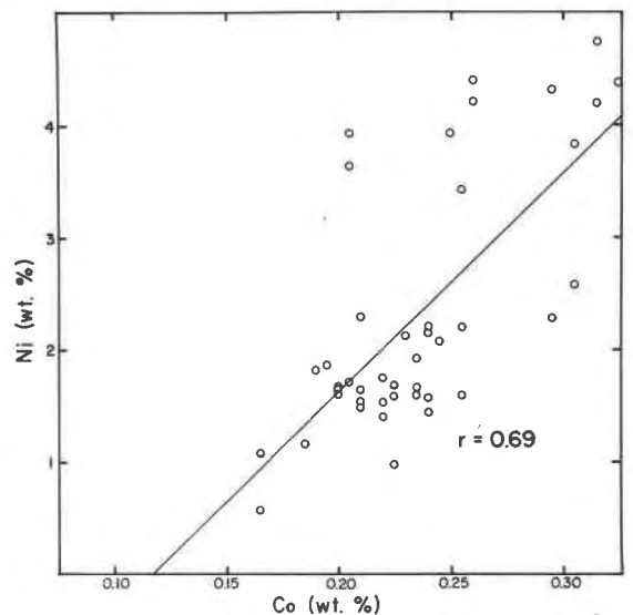
Fig. 3. Nickel and cobalt contents of 32 grains of low-Ni and 11 grains of high-Ni suessite from the North Haig ureilite as determined by electron microprobe analysis. Symbols as in Fig. 2.
