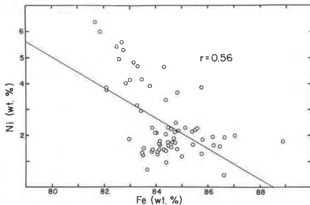
Fig. 2. Nickel and iron contents of 47 grains of low-Ni and 20 grains of high-Ni suessite from the North Haig ureilite, as determined by electron microprobe analysis. Boundary between low- and high-Ni suessite is at ~2.7% Ni. Diagonal line is a multivariate best-fit regression line; r = statistical correlation coefficient.
