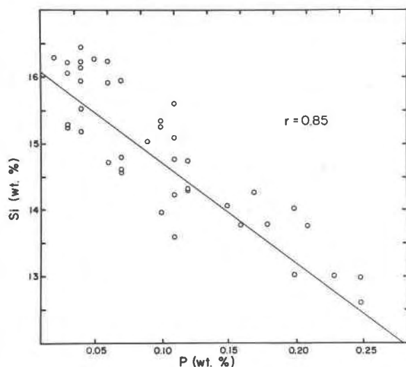
Fig. 4. Silicon and phosphorous contents of 26 grains of low-Ni and 15 grains of high-Ni suessite from the North Haig ureilite as determined by electron microprobe analysis. Symbols as in Fig. 2.
