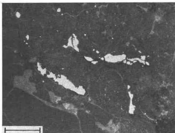
Fig. 1. Suessite (white) as vein fillings and blebs in the North Haig ureilite. Silicates (olivine, pigeonite) are gray; carbonaceous matrix is black. Hydrous ferric oxide veins (light gray) are of terrestrial weathering origin. Reflected, plane polarized light. Scale bar equals 100 \mu\text{m} .
