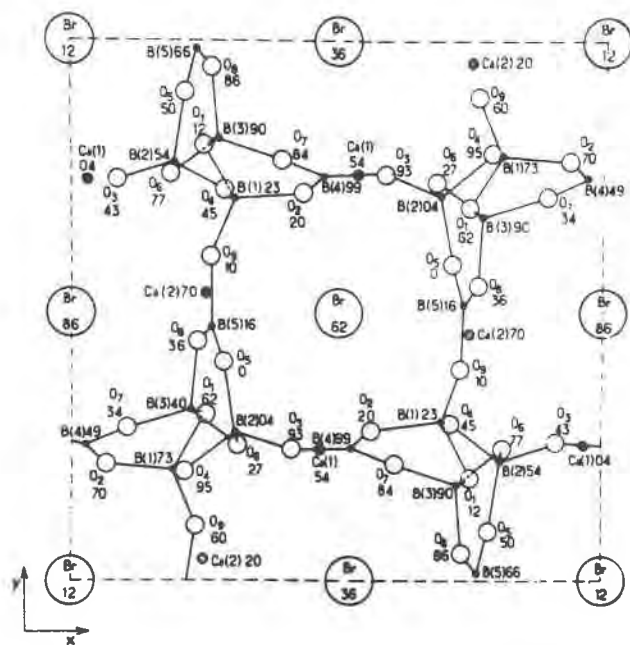
Fig. 7. Crystal structure of \text{Ca}_2\text{B}_5\text{O}_9\text{Br} (isostructural with \text{Ca}_2\text{B}_5\text{O}_9\text{Cl} ) projected down the c axis (after Lloyd et al. 1973).
