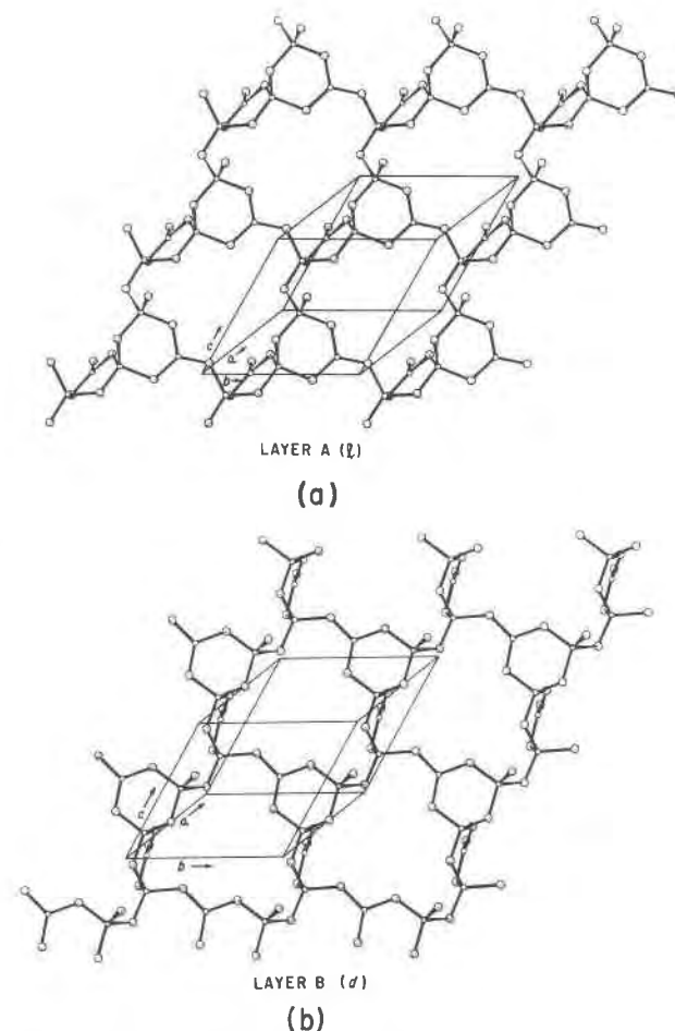
Fig. 3. Two stereoisomeric pentaborate layers, (a) and (b), formed by pentaborate polyanions in l and d configurations respectively as found in parahilgardite parallel to the (100) plane (after Wan and Ghose, in prep.).
