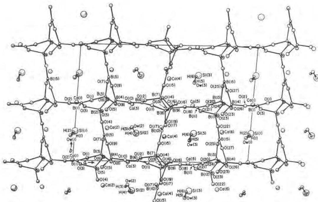
Fig. 8. Crystal structure of parahilgardite projected down the c axis (after Wan and Ghose, in prep.).
