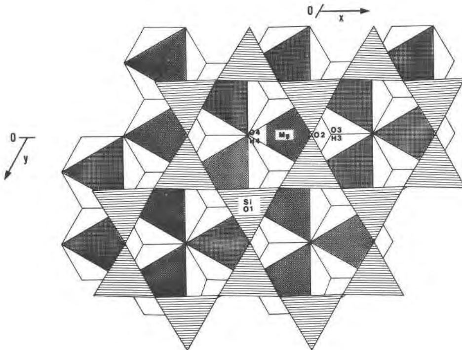
Fig. 2. 1 : 1 layer of lizardite 1T, viewed along [001].
