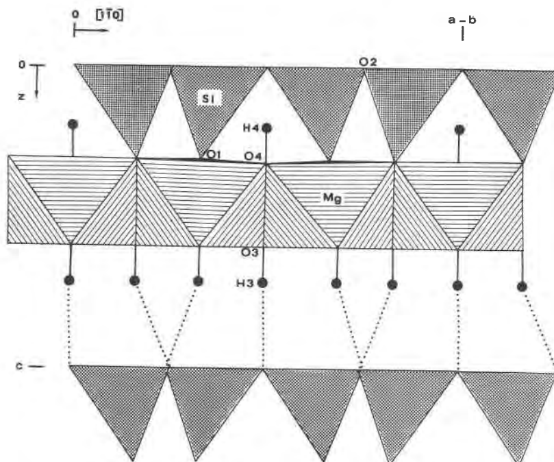
Fig. 3. Crystal structure of lizardite 1T, viewed along [110]. Dotted lines represent hydrogen bonds.
