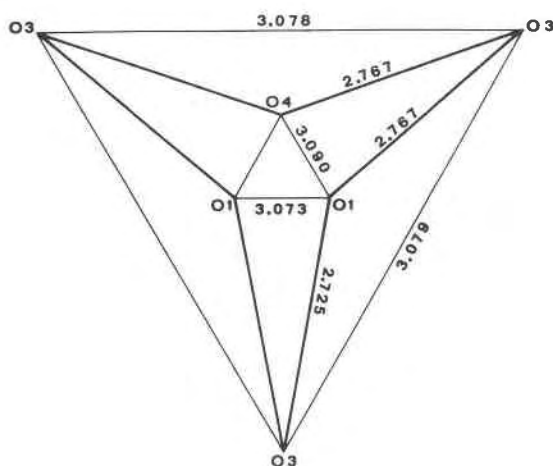
Fig. 4. The octahedral site, represented by Schlegel diagram. Heavy lines represent shared edges.
