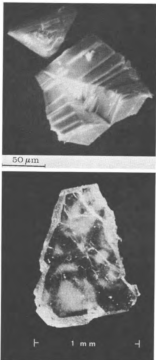
Fig. 1. a) Crystals of lizardite 1T, observed by SEM; b) Photograph of a large crystal of lizardite 1T.
