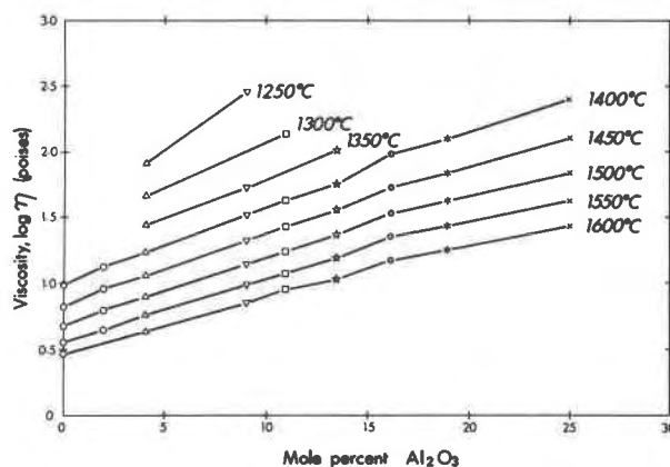
Fig. 2. Plot of log η vs. mole% Al 2 O 3 . Isotherms at 50°C intervals between 1250–1600°C.
