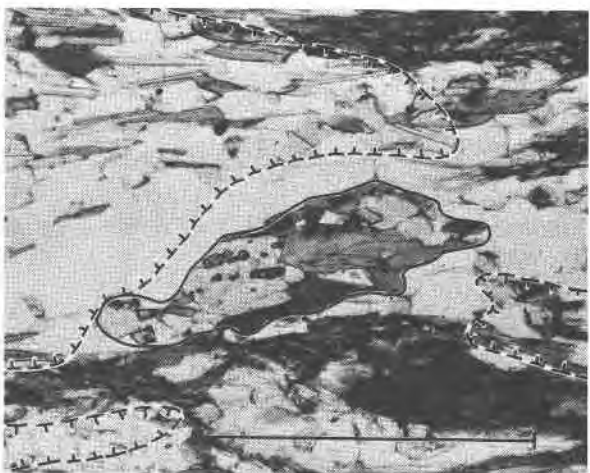
Fig. 2. Muscovite-free, biotite-rich, plagioclase-rich pseudomorph after staurolite (52% biotite, 38% plagioclase, 10% quartz). The pseudomorph boundary is shown by a solid line. Light gray grains are stained plagioclase. High relief grains within plagioclase in the pseudomorph are staurolite remnants. The matrix/muscovite-free mantle boundary is marked by the dashed line. The tick marks are on the matrix side of the line. The scale bar is 1 mm.
