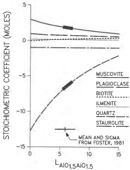
Fig. 6. Stoichiometric coefficients ( R_K ) calculated by the model for staurolite dissolving in a matrix of muscovite, biotite, plagioclase, quartz and ilmenite as a function of the aluminum diffusion coefficient. The heavy portion of the muscovite and the quartz curves show where the quartz to muscovite ratio in the model is within one standard deviation of the observed ratio. The mean and standard deviation of the aluminum diffusion coefficient calculated by Foster (1981) is also shown.
