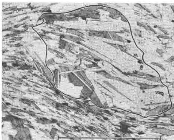
Fig. 1. Muscovite-rich pseudomorph after staurolite (51% muscovite, 26% biotite, 14% plagioclase, 8% quartz, 1% ilmenite). The boundary of the pseudomorph is shown by a solid line. The small, high relief blebs in muscovite in the pseudomorph are remnants of staurolite. The scale bar is 1 mm.
