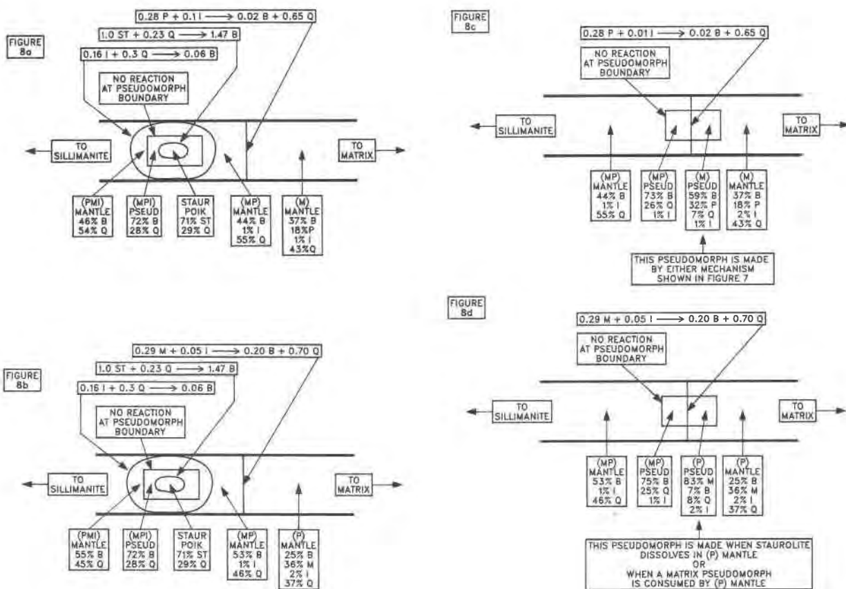
Fig. 8. Local reactions and mineral modes calculated by the model for the formation of muscovite-free, plagioclase-free, biotite-rich pseudomorphs after staurolite. Mineral abbreviations same as in Fig. 7. Minerals not present are shown in parentheses.
