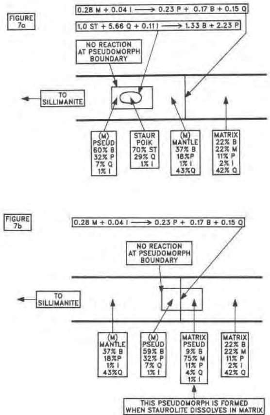
Fig. 7. Local reactions and mineral modes calculated by the model for the formation of muscovite-free, biotite-rich, plagioclase-rich pseudomorphs after staurolite. (M) stands for muscovite-free. M=muscovite, B=biotite, P=plagioclase, I=ilmenite, Q=quartz, St=staurolite
