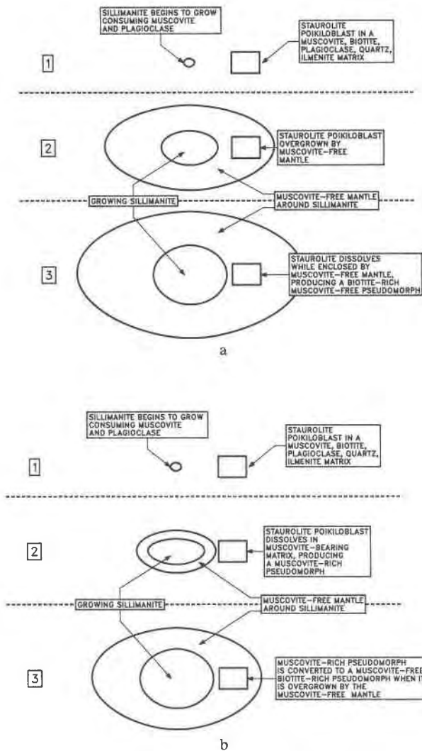
Fig. 4. Mechanisms for the development of muscovite-free, biotite-rich, plagioclase-rich pseudomorphs.
