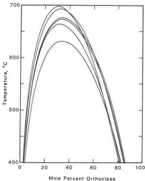
Fig. 5. Calculated solvi at 1 bar based on the phase-equilibrium studies (in order of decreasing critical temperature) of Orville (1963), Luth and Tuttle (1966), Seck (1972), Smith and Parsons (1974), Goldsmith and Newton (1974), and Lagache and Weisbrod (1977).
