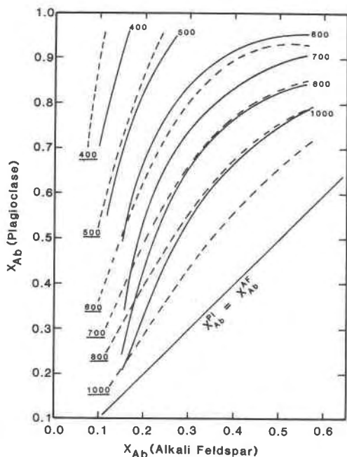
Fig. 8. The distribution of \text{NaAlSi}_3\text{O}_8 component between alkali feldspar and plagioclase at 1 bar and in the range 400–1000°C. The present formulation given by equation 5 is represented by solid curves and that of Stormer (1975, Equation 18) by dashed curves. The temperatures of the isotherms for Stormer are underlined. The distribution of isotherms in the present formulation is complicated at low temperatures (<560°C) by the presence of a solvus in the plagioclase binary.
