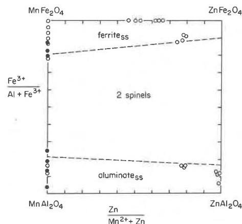
Fig. 2. The composition space \text{MnAl}_2\text{O}_4 – \text{MnFe}_2\text{O}_4 – \text{ZnAl}_2\text{O}_4 – \text{ZnFe}_2\text{O}_4 with spinel analyses plotted. Symbols and references the same as for Fig. 1, with additional references: Palache (1935), Kayupova et al. (1970), Vogel et al. , (1976). Spinel with >0.05 Mg, \text{Fe}^{2+} , \text{Mn}^{3+} or Ti per four oxygens are excluded.
