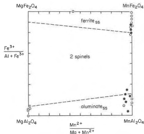
Fig. 1. The composition space \text{MnAl}_2\text{O}_4 – \text{MnFe}_2\text{O}_4 – \text{MgAl}_2\text{O}_4 – \text{MgFe}_2\text{O}_4 with spinel analyses plotted. Closed circles: data on Bald Knob spinels; open circles: data from other occurrences. References: Ross and Kerr (1932) Stillwell and Edwards (1951), Lee (1968), Kuno (1960), Deer et al. , (1962), Berg (1976), Bowman (1978), Carvalho (1978), Chopin (1978), Fukuoka and Hirowatari (1980), Fukuoka (1981). Spinel with >0.05 Zn, \text{Fe}^{2+} , \text{Mn}^{3+} or Ti per four oxygens are excluded.
