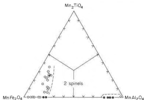
Fig. 3. The composition space \text{MnAl}_2\text{O}_4 – \text{MnFe}_2\text{O}_4 – \text{Mn}_2\text{TiO}_4 with spinel analyses plotted. Symbols and references the same as for Figure 1. Spinel with >0.30 \text{ Fe}^{2+} , or 0.10 \text{ Mg} , \text{Zn} , \text{Mn}^{3+} are excluded.
