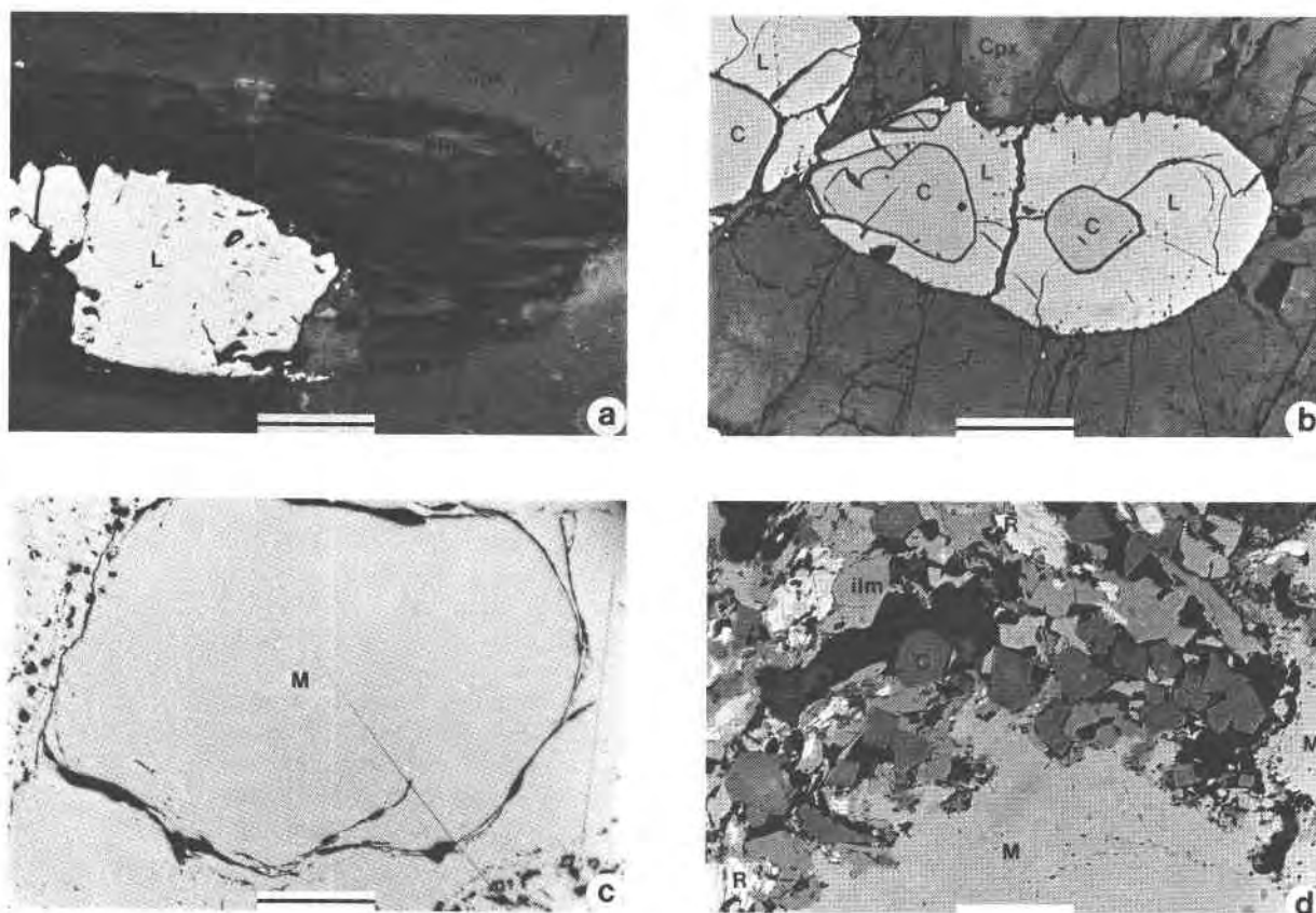
Fig. 1. (a) Lindsleyite (L) enclosed in phlogopite (Phl) and surrounded by chrome diopside (Cpx) and K-richterite (Ric). Sample BD-3096, Bultfontein. Mixed reflected and transmitted light in oil-immersion. Scale bar = 0.1mm. (b) Lindsleyite (L) enclosing chrome spinel (C) and surrounded by chrome diopside (Cpx). Sample JIG-360, Bultfontein. Reflected light in air. Scale bar = 0.2mm. (c) Mathiasite (M) exhibiting typical curvilinear cracks and incipient decomposition (upper left and lower right). Sample JF18-1, Jagersfontein. Reflected light in air. Scale bar = 0.2mm. (d) Mathiasite (M) decomposing to chrome spinel (C) + ilmenite (ilm) + rutile (R). The rutile contains oriented sigmoidal lamellae of ilmenite and the dark interstitial groundmass is composed of phlogopite (Phl), calcite, and sphene. Sample JF-111, Jagersfontein. Reflected light in oil-immersion. Scale bar = 0.1mm.
