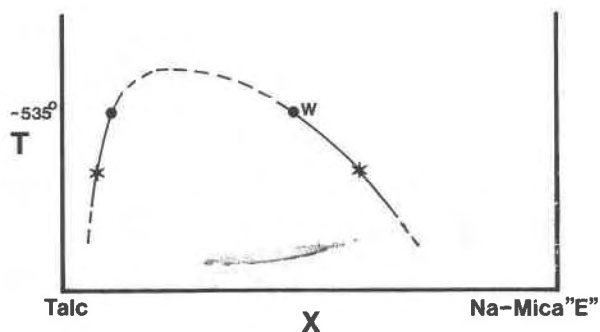
Fig. 9. A schematic temperature-composition ( T - X ) diagram showing the talc-wonesite miscibility gap. The Na-mica composition "E" is shown in Figure 8. Circles represent the bulk wonesite ("W") and talc compositions obtained by microprobe analysis by Spear et al. (1981); these are primary crystallization compositions representing a temperature of approximately 535°C. The compositions "*" were derived from the individual talc and wonesite exsolution lamellae by analytical TEM methods, as discussed in the text. The analyses are consistent with a miscibility gap skewed strongly toward talc.
