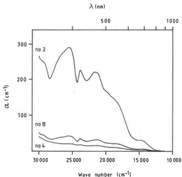
Fig. 4. Room temperature E\perp X absorption spectra of samples 2, 4 and 8, with [\text{Fe}_{\text{IV}}^{3+}][\text{Mn}_{\text{VI}}^{2+}] concentration products of [1.23][3.43] , [0.44][0.45] and [0.76][0.69] g-atom l^{-1} respectively. \alpha as in Fig. 2.
