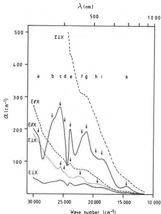
Fig. 2. Room temperature E \parallel X and E \perp X absorption spectra of sample 1 (---), sample 8 (—) and E \perp X spectrum of synthetic Fe_{IV}^{3+} -phlogopite (···). \alpha = absorbance/sample thickness (cm). For the reverse pleochroic sample 8, letters a, b, . . . and arrows indicate absorption bands assigned in Table 3. Arrows at the spectra of the synthetic sample and the normal pleochroic sample 1 denote bands which occur at the same energies as bands in the reverse pleochroic samples.
