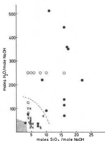
Fig. 1. Syntheses from \text{SiO}_2 - \text{NaOH} - \text{H}_2\text{O} suspensions at 100°C or 150°C. ● kenyaite (100°C), ○ kenyaite (150°C), × magadiite (100°C), ■ "octosilicate"; (100°C), □ unidentified phase (150°C), stippled area: makatite and "octosilicate" field (100°C), dashed line is the speculated stability field boundary between magadiite and kenyaite.
