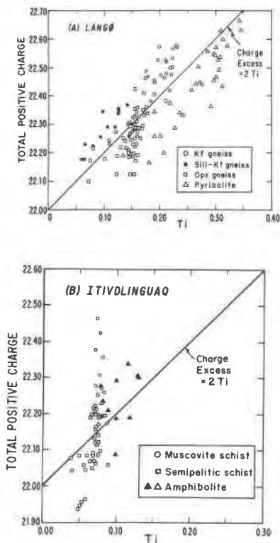
Fig. 3. Calculated total positive charge and Ti-content in biotite from Langø (a) and Itivdlinguaq (b), with formula proportions based on the 7 cation normalization (A).
