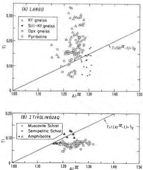
Fig. 2. Ti- and Al IV -contents of biotite from West Greenland with formula proportions based on the 11 oxygen normalization (B).
