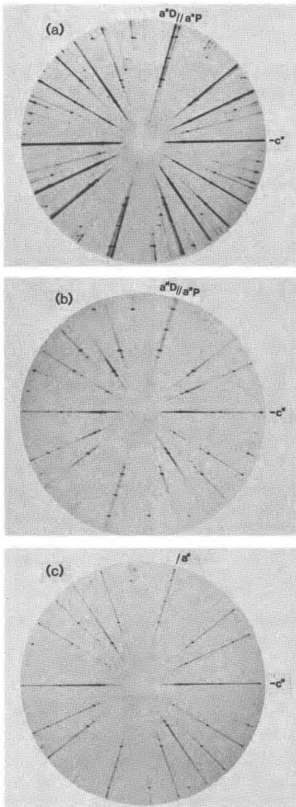
Fig. 1. b -axis precession X-ray photographs of the Mabuki pyroxene (a) prior to any experiments, (b) after 15 minutes at 1150^\circ\text{C} , and (c) after 25 minutes at 1250^\circ\text{C} (all at 25 kbar).
