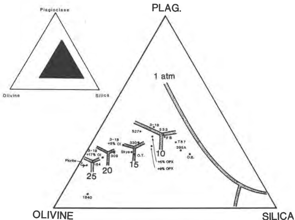
Fig. 2. Pseudo-liquidus phase diagram projected from clinopyroxene. See text for discussion. The apices of the triangle are: (top) AN_{65}OL_{10}SIL_{25} (left) OL_{60}AN_{15}SIL_{25} (right) SIL_{75}AN_{15}OL_{10} . Details of the projection method are given in Elthon (1983). 1 atm phase equilibria are from Walker et al. (1979).
