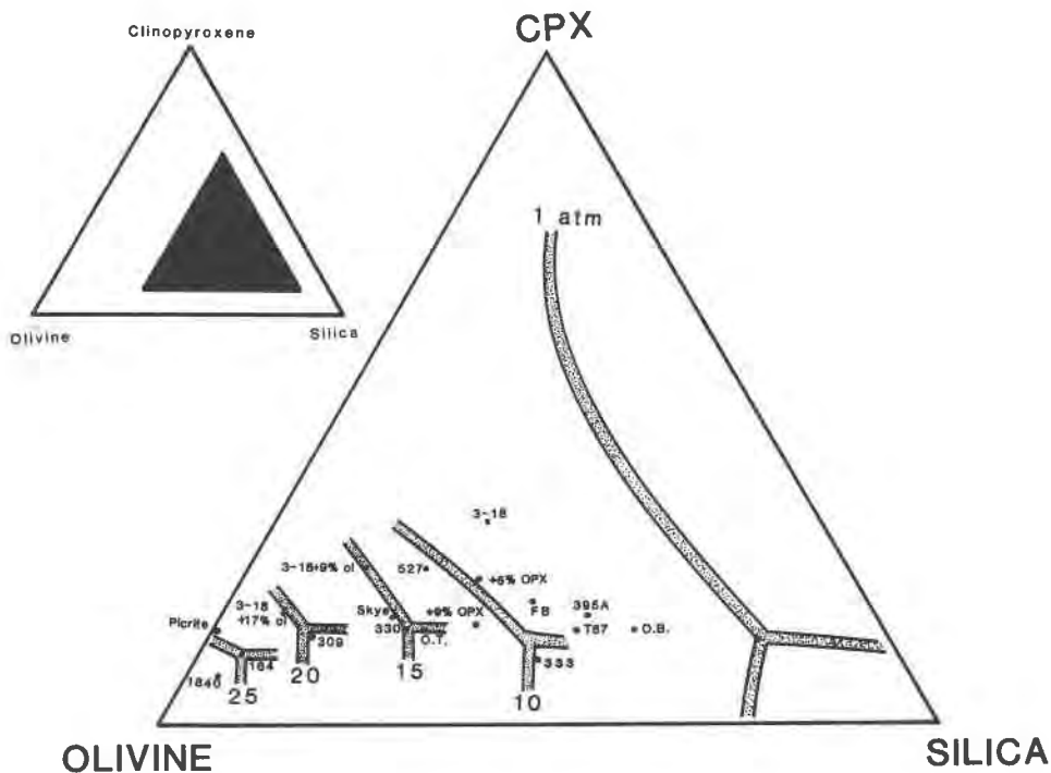
Fig. 3. Pseudo-liquidus phase diagram projected from anorthite. See text for discussion. The apices of the triangle are: (top) CPX_{60}OL_{10}SIL_{30} (left) OL_{60}CPX_{10}SIL_{30} (right) SIL_{80}CPX_{10}OL_{10} . 1 atm phase equilibria are from Walker et al. (1979).
