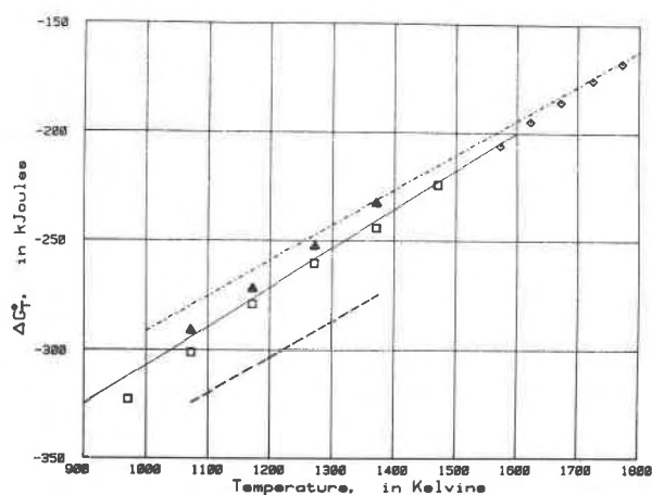
Fig. 2. Change in the Gibbs free energy versus temperature for the reaction 2Ni + SiO_2 + O_2 = Ni_2SiO_4 . Solid triangles, Taylor and Schmalzried (1964); rectangles, Burdese et al. (1963); open diamonds, Campbell and Roeder (1968); dashed line Lebedev and Levitskii (1961); solid line, calculated from calorimetric data; dot-dash line calculated from equation of Kother and Muller (1978).
