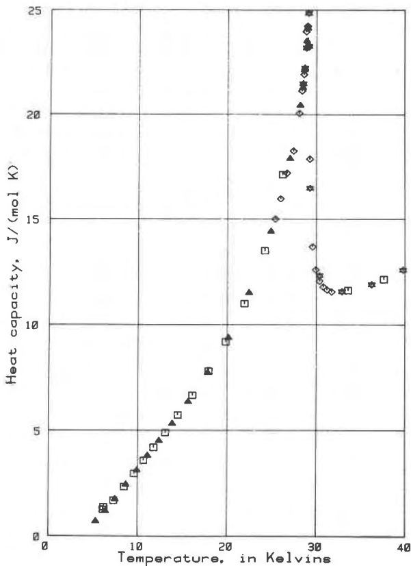
Fig. 1. Experimental molar heat capacities of \text{Ni}_2\text{SiO}_4 -olivine in the neighborhood of the Néel temperature. Open rectangles, series 1; open diamonds, series 2; solid triangles, series 1a; open stars, series 2a.
