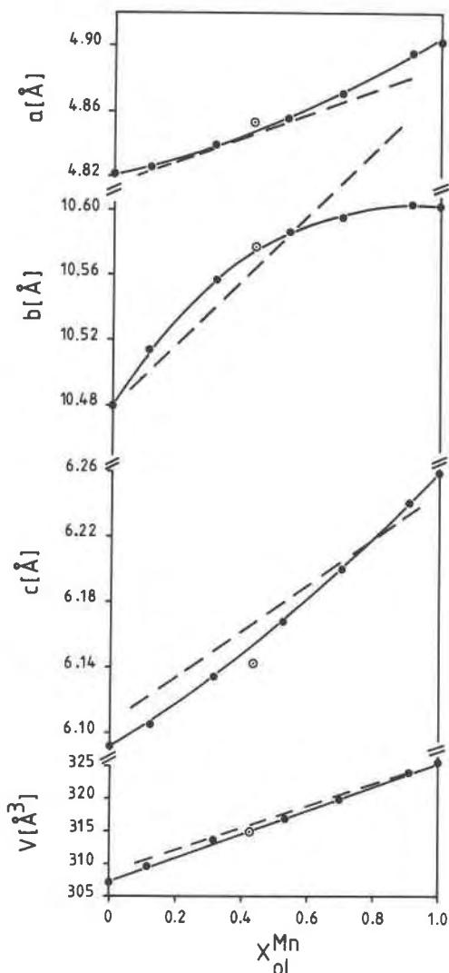
Fig. 1. Cell parameter variations in the (Fe,Mn) 2 SiO 4 solid solution series. Solid dots are synthetic samples, open circles are natural samples (unheated). Dashed line calculated cell parameter variations from regression equation (Lumpkin and Ribbe, 1983).
